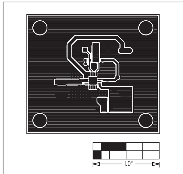
Figure 3. MAX16836 EV Kit PCB Layout—Component Side
