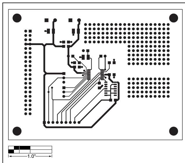
Figure 3. MAX1132 EV Kit PCB Layout—Component Side
