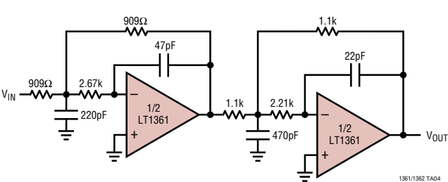
1MHz, 4th Order Butterworth Filter
