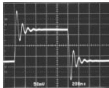
Small-Signal Transient ( A_V = -1 , C_L = 500\text{pF} )
