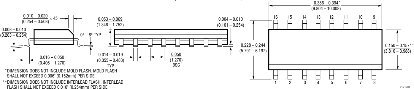
S Package 16-Lead Plastic Small Outline (Narrow 0.150) (LTC DWG # 05-08-1610)
