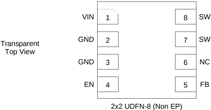
Figure 3. 34726 Pin Connections
