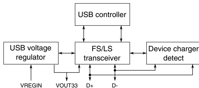
Figure 3-47. USB Subsystem Overview
