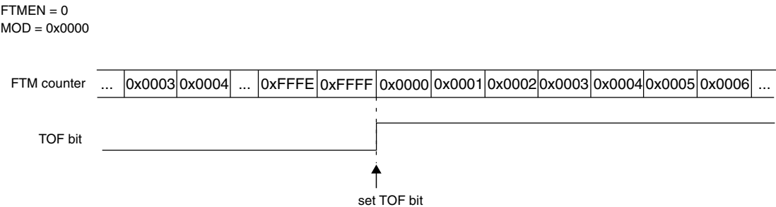
Figure 37-172. Example when the FTM counter is free running
