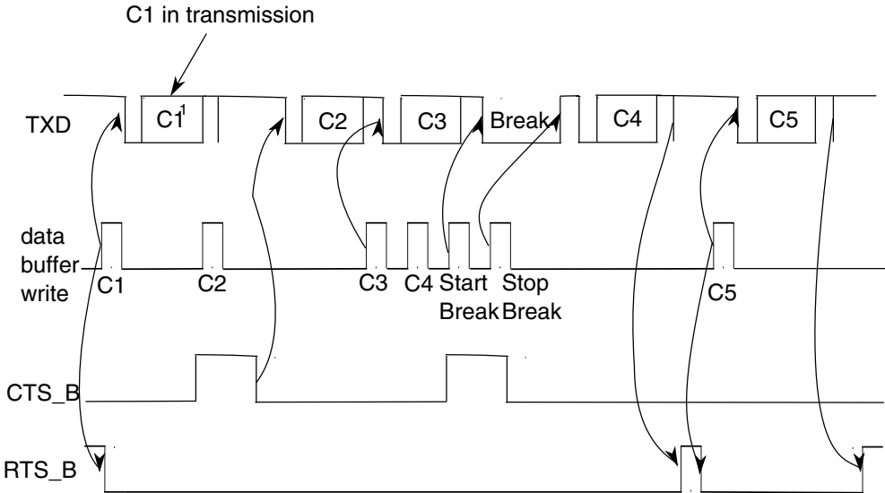
Figure 48-295. Transmitter RTS and CTS timing diagram
