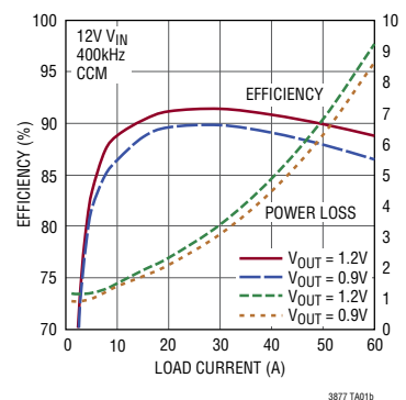
Efficiency and Power Loss vs Load Current
