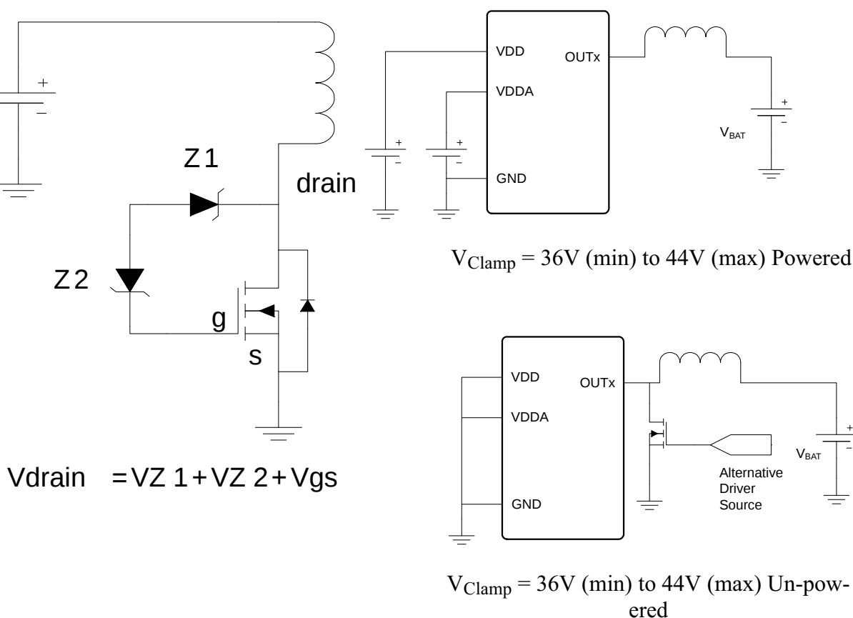
Figure 22. Output Clamp
