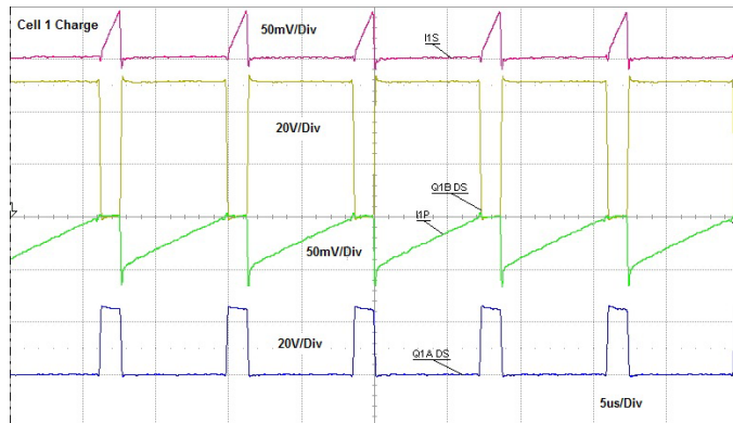
Figure 24. 12 Cells Charge Waveforms
