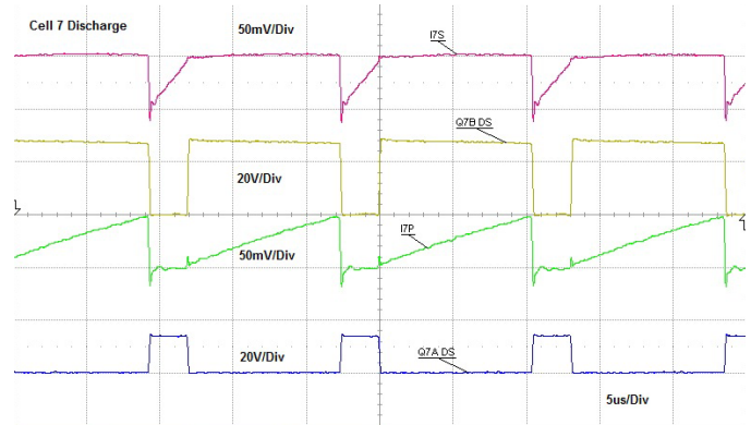
Figure 25. 6 Cells Discharge Waveforms
