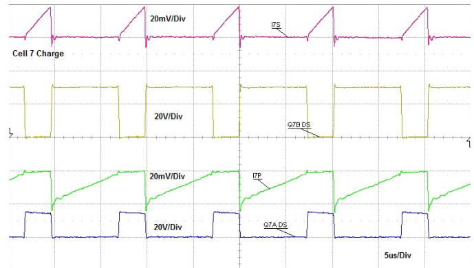
Figure 26. 6 Cells Charge Waveforms
