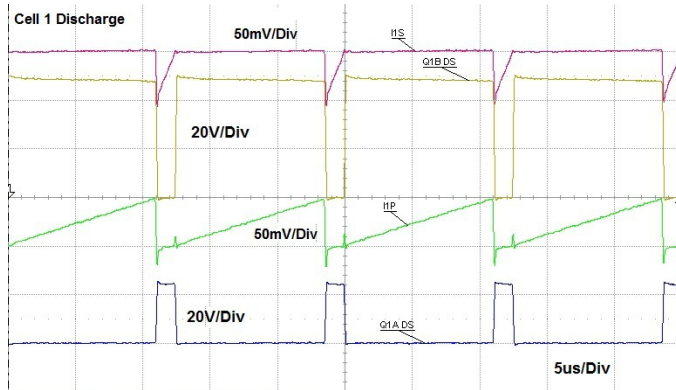
Figure 23. 12 Cells Discharge Waveforms
