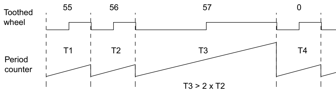
Figure 21-45. Gap Verification Criteria For a 60-2 Toothed Wheel
