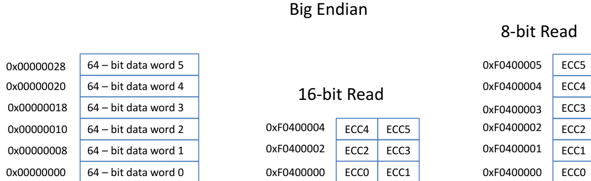
Figure 5-1. ECC Organization for Program Flash (144-Bits Wide)
