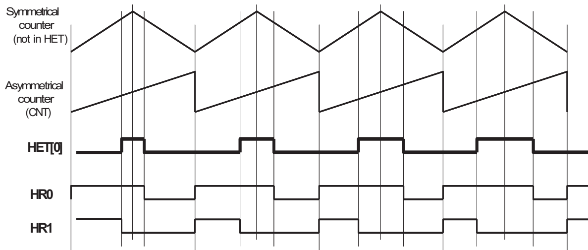
Figure 21-14. Symmetrical PWM with XOR-sharing Output
