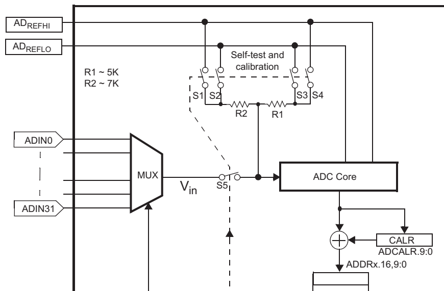
Figure 20-13. Self-Test and Calibration Logic
