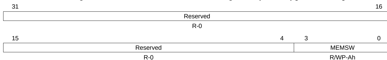
Figure 2-46. Bus Matrix Module Control Register 1 (BMMCR) [offset = C4h]
