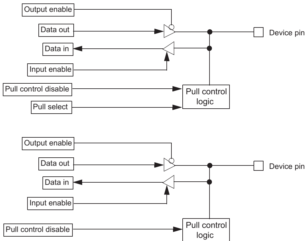
Figure 27-32. GPIO Functionality
