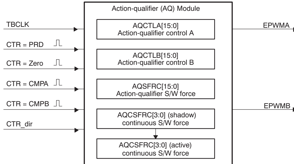
Figure 17-18. Action-Qualifier Submodule Inputs and Outputs
