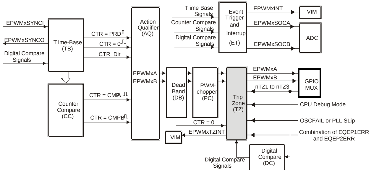
Figure 17-35. Trip-Zone Submodule
