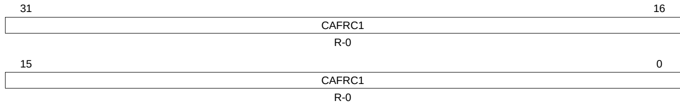
Figure 13-20. RTI Capture Free Running Counter 1 Register (RTICAFRC1) [offset = 40h]
