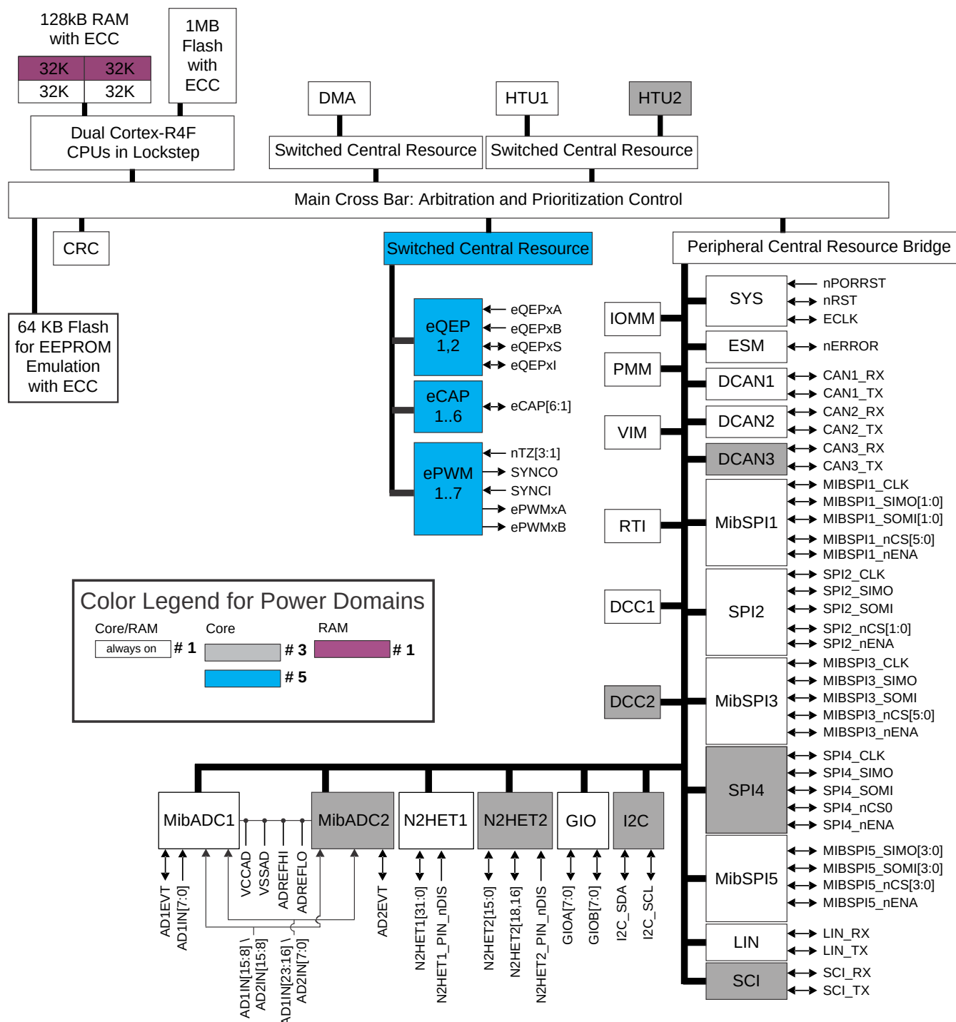
Figure 1-1. Block Diagram
