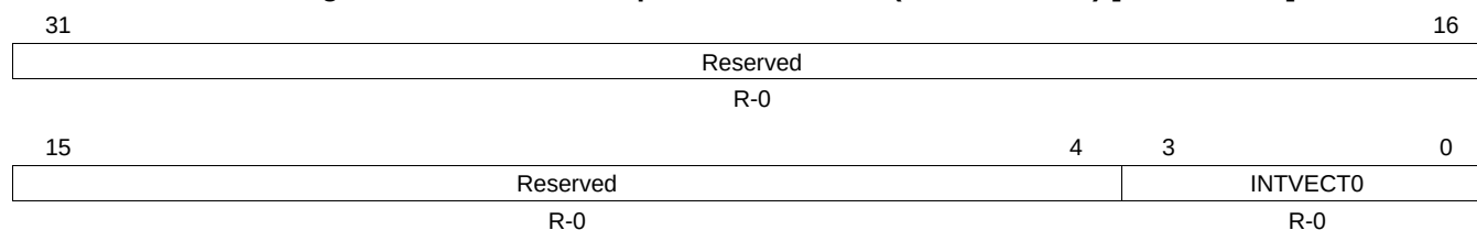
Figure 27-15. SCI Interrupt Vector Offset 0 (SCIINTVECT0) [offset = 20h]
