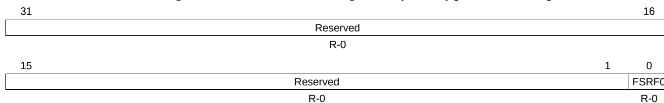
Figure 7-8. Fail Status Fail Register 0 (FSRF0) [offset = 0190h]
