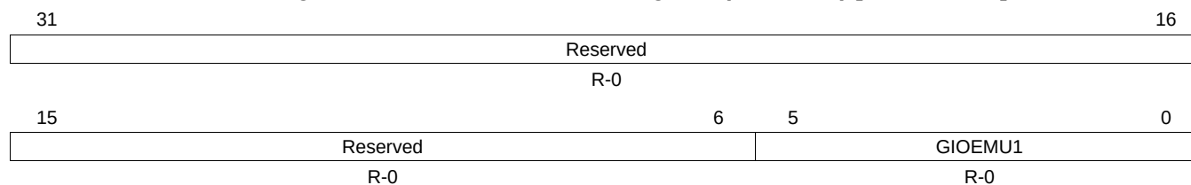
Figure 23-15. GIO Emulation 1 Register (GIOEMU1) [offset = 2Ch]
