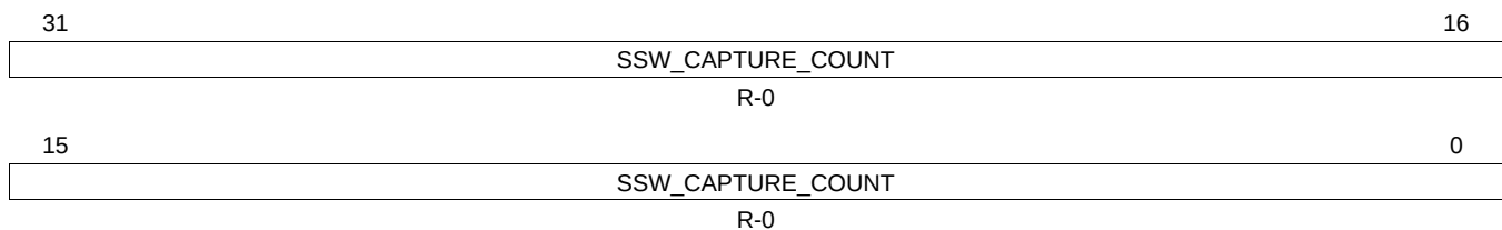
Figure 10-7. SSW PLL BIST Control Register 2 (SSWPLL2) [offset = FF28h]
