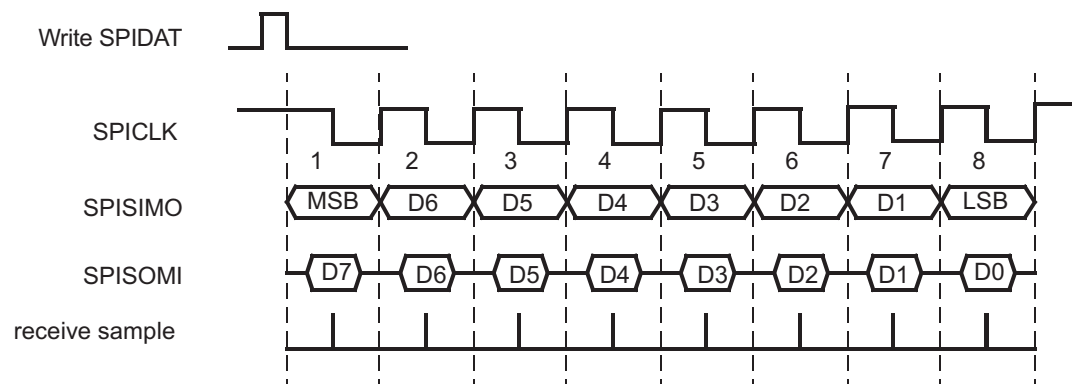
Figure 25-11. Clock Mode with Polarity = 1 and Phase = 1
