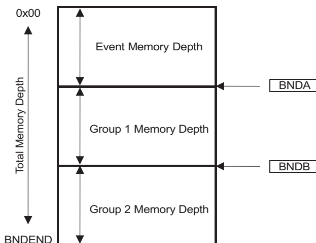
Figure 20-3. FIFO Implementation
