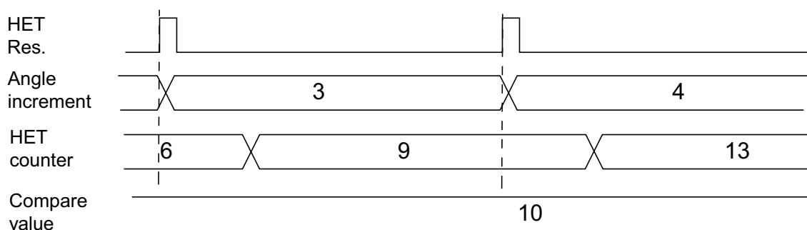
Figure 21-53. Compare Without ACMP Instruction
