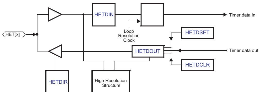
Figure 21-8. I/O Control
