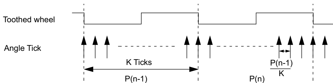
Figure 21-37. Angle Tick Generation Principle
