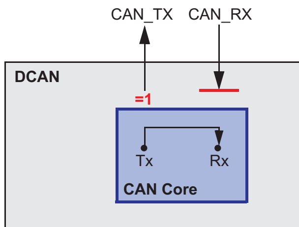
Figure 24-18. CAN Core in Loop Back Combined with Silent Mode
