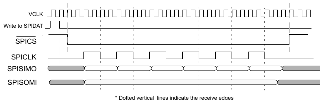
Figure 25-82. SPI/MibSPI Pins During Master Mode 4-pin with \overline{\text{SPIC}}\text{S} Configuration
