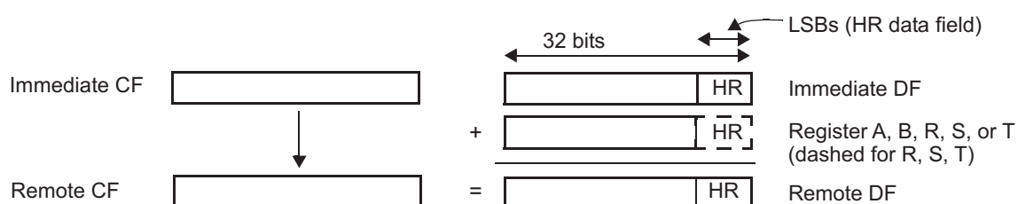
Figure 21-173. RADM64 Add and Move Operation
