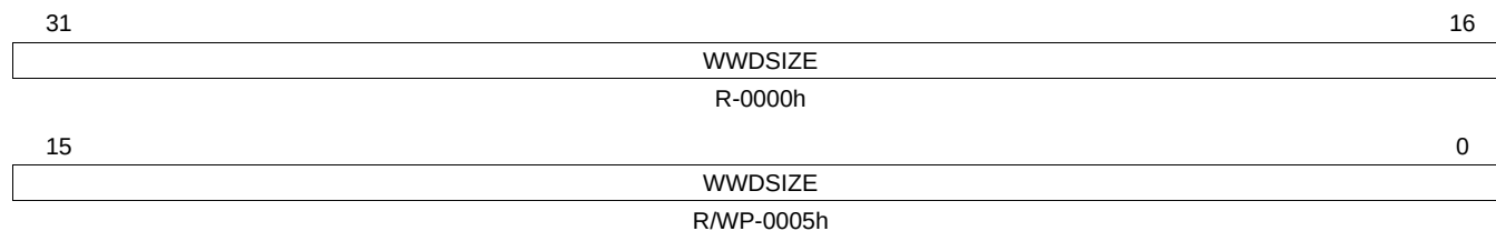
Figure 13-39. Digital Windowed Watchdog Window Size Control (RTIWWDSIZECTRL) [offset = A8h]
