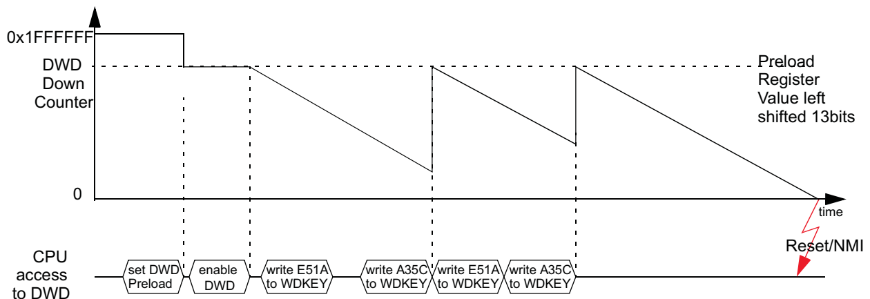
Figure 13-5. DWD Operation
