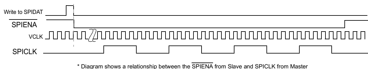
Figure 25-86. SPI/MibSPI Pins During Slave Mode 4-pin with \overline{\text{SPIENA}} Configuration
