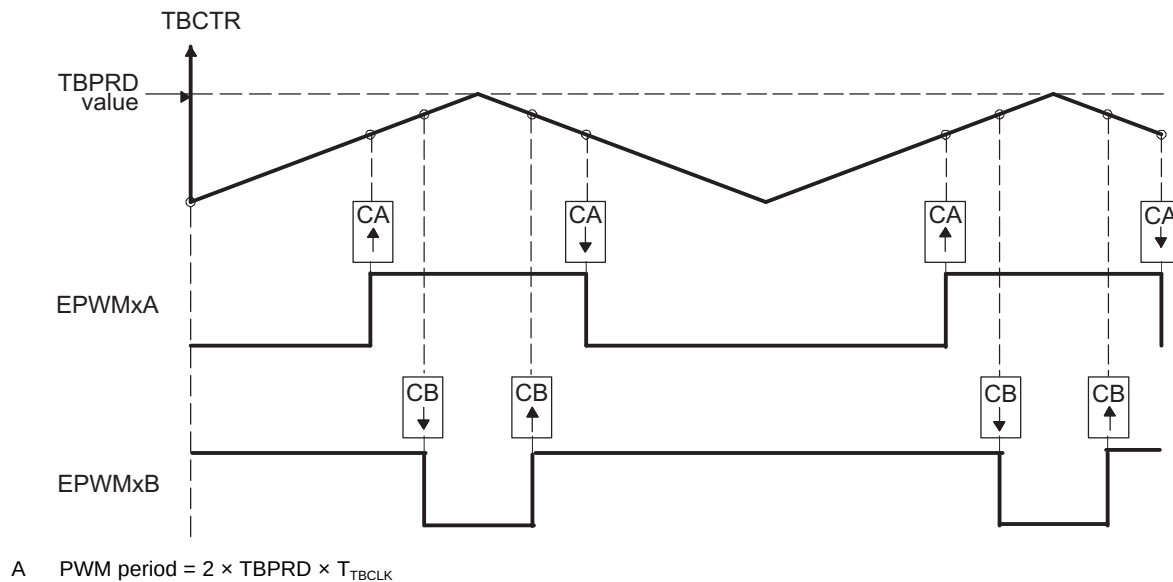
Figure 17-25. Up-Down-Count, Dual Edge Symmetric Waveform, With Independent Modulation on EPWMxA and EPWMxB — Complementary
