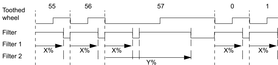
Figure 21-48. Filtering During Singularity Tooth
