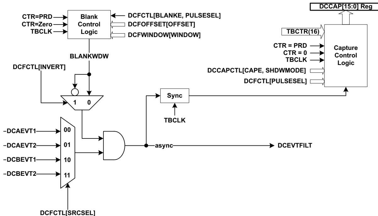
Figure 17-49. Event Filtering
