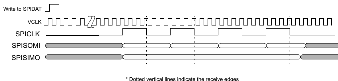
Figure 25-85. SPI/MibSPI Pins During Slave Mode 3-pin Configuration
