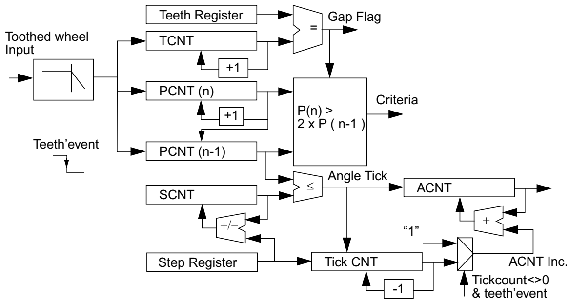
Figure 21-38. New Angle Tick Generation Architecture
