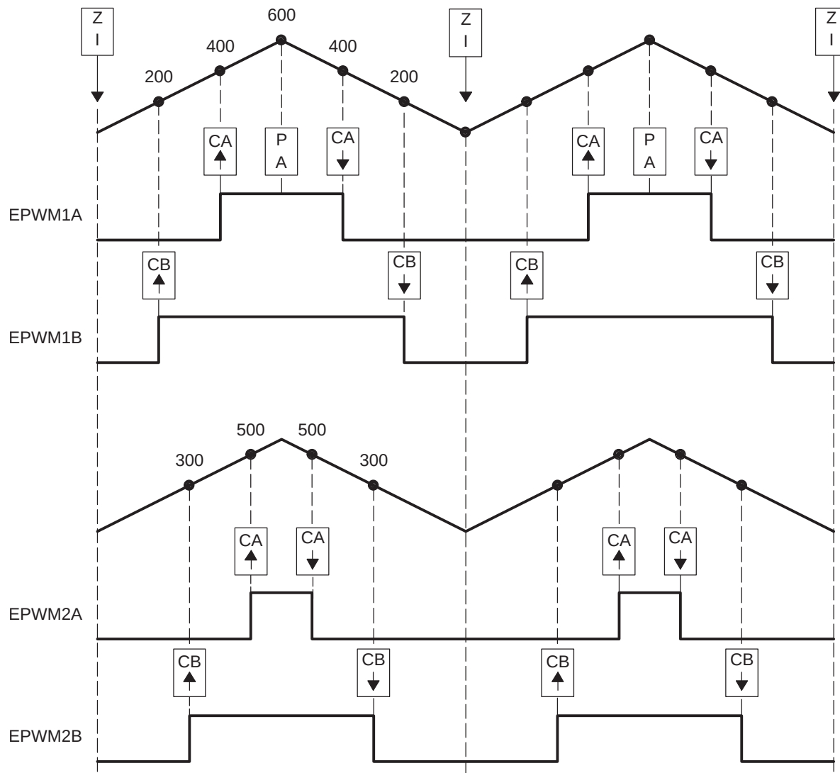
Figure 17-56. Buck Waveforms for Figure 17-55 (Note: F_{PWM2} = F_{PWM1} )
