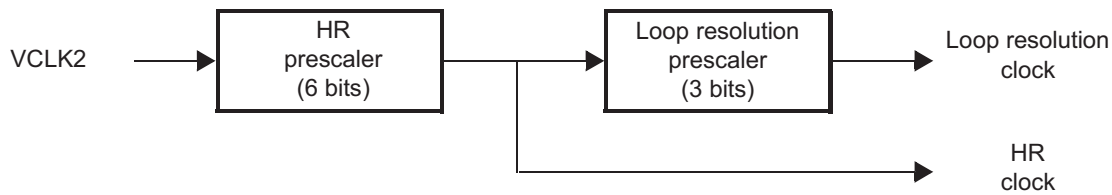
Figure 21-7. Prescaler Configuration
