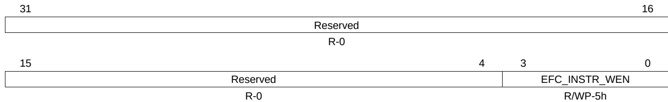
Figure 2-61. EFUSE Controller Control Register (EFC_CTLREG) [offset = ECh]
