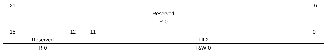
Figure 21-107. HWAG Filter Register 2 (HWAFIL2)
