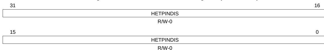
Figure 21-88. N2HET Pin Disable Register (HETPINDIS)
