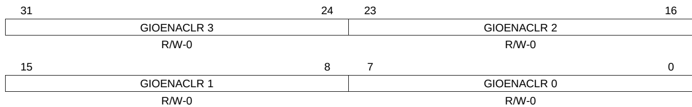
Figure 23-9. GIO Interrupt Enable Clear Register (GIOENACLR) [offset = 14h]
