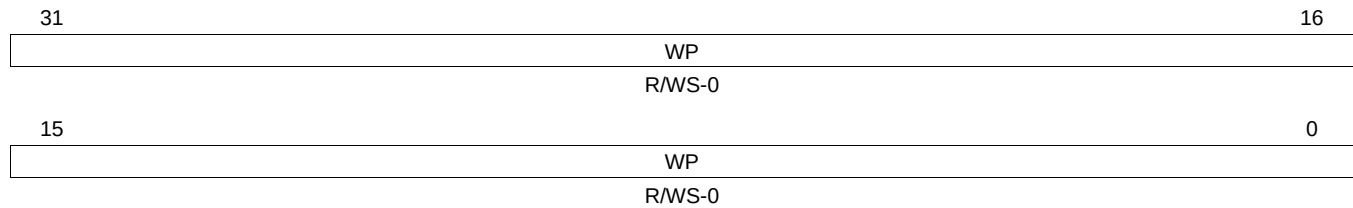
Figure 22-34. Watch Point Register (HTU WPR) [offset = 58h]
