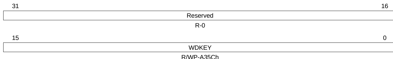
Figure 13-36. RTI Watchdog Key Register (RTIDWDKEY) [offset = 9Ch]
