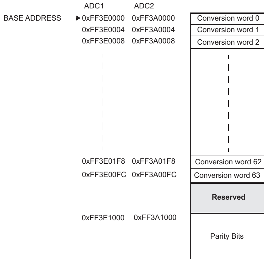
Figure 20-18. ADC Memory Map in Parity Test Mode
