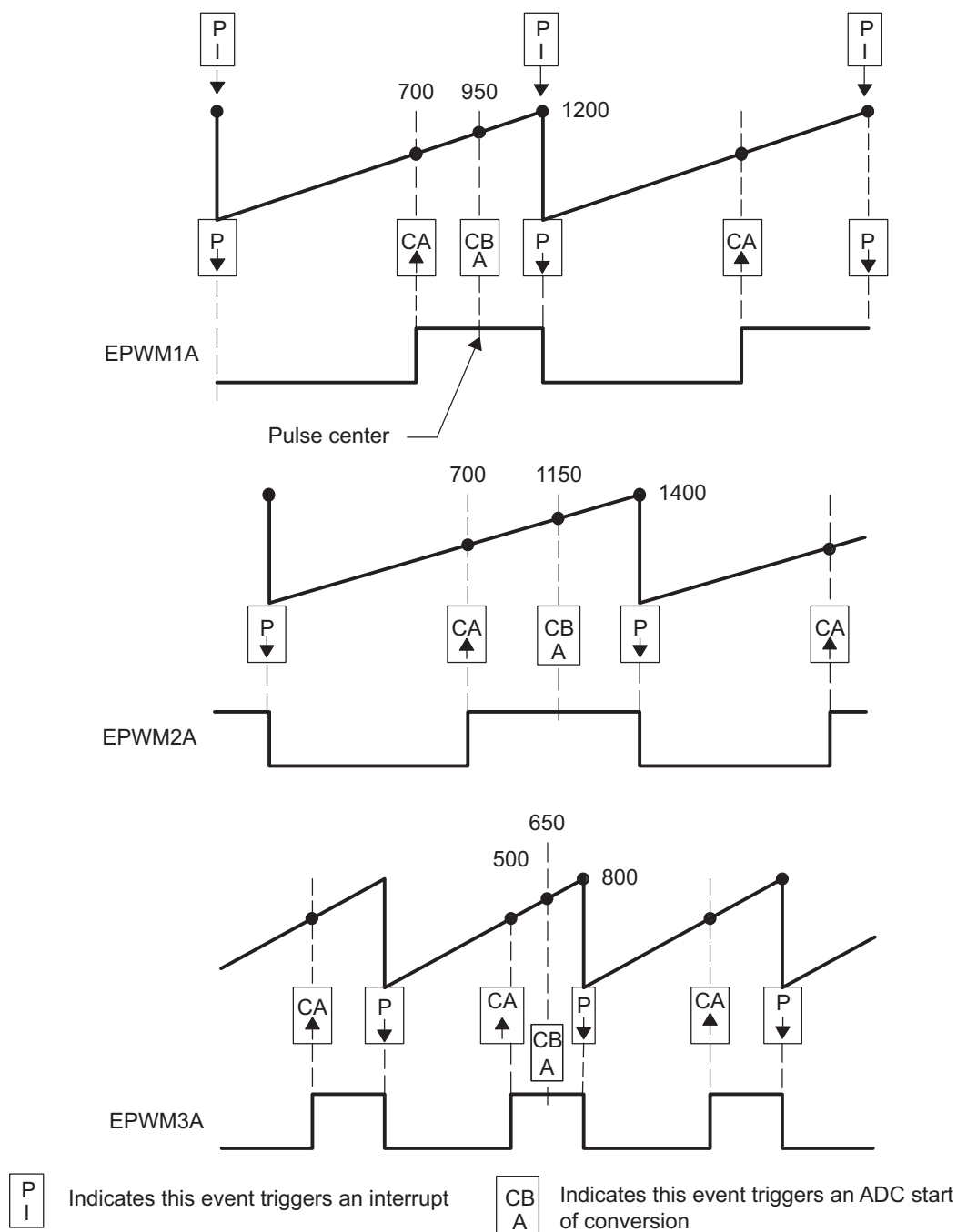
Figure 17-54. Buck Waveforms for Figure 17-53 (Note: Only three bucks shown here)
