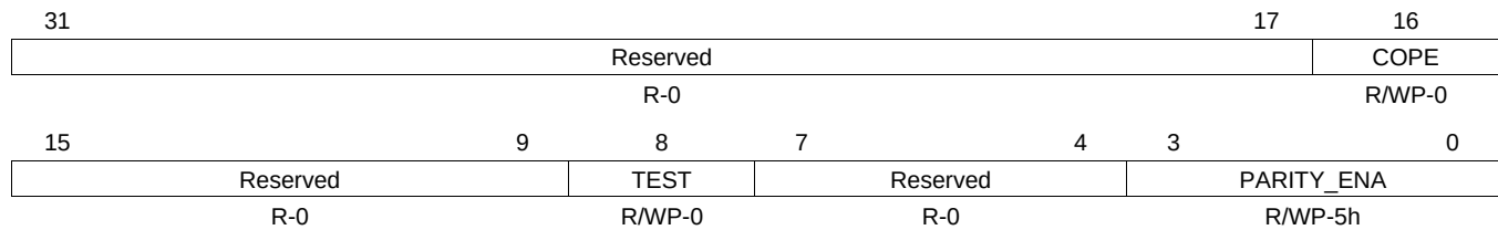
Figure 22-37. Parity Control Register (HTU PCR) [offset = 64h]
