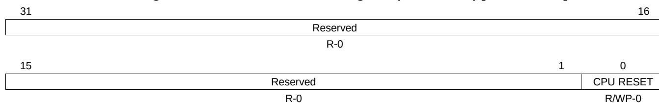
Figure 2-47. CPU Reset Control Register (CPURSTCR) [offset = CCh]
