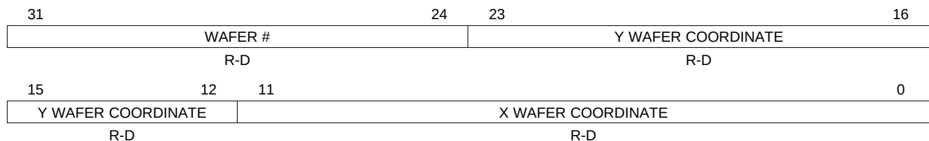
Figure 2-62. Die Identification Register, Lower Word (DIEIDL_REG0) [offset = F0h]
