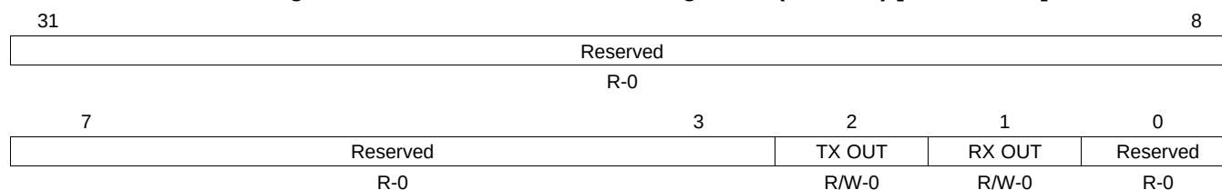
Figure 26-45. SCI Pin I/O Control Register 3 (SCIPIO3) [offset = 48h]
