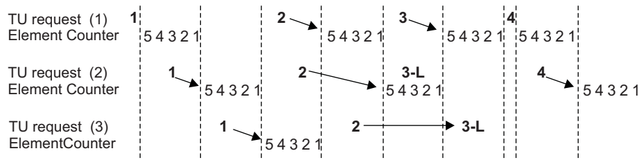
Figure 22-9. Timing Example Including Lost Requests
