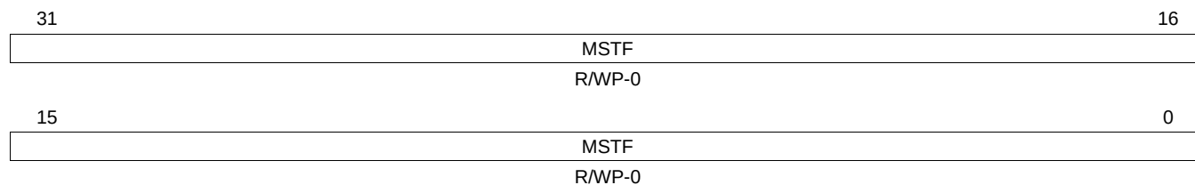
Figure 2-28. Memory Self-Test Fail Status Register (MSTFAIL) [offset = 64h]
