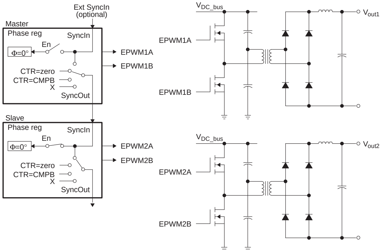
Figure 17-57. Control of Two Half-H Bridge Stages ( F_{PWM2} = N \times F_{PWM1} )
