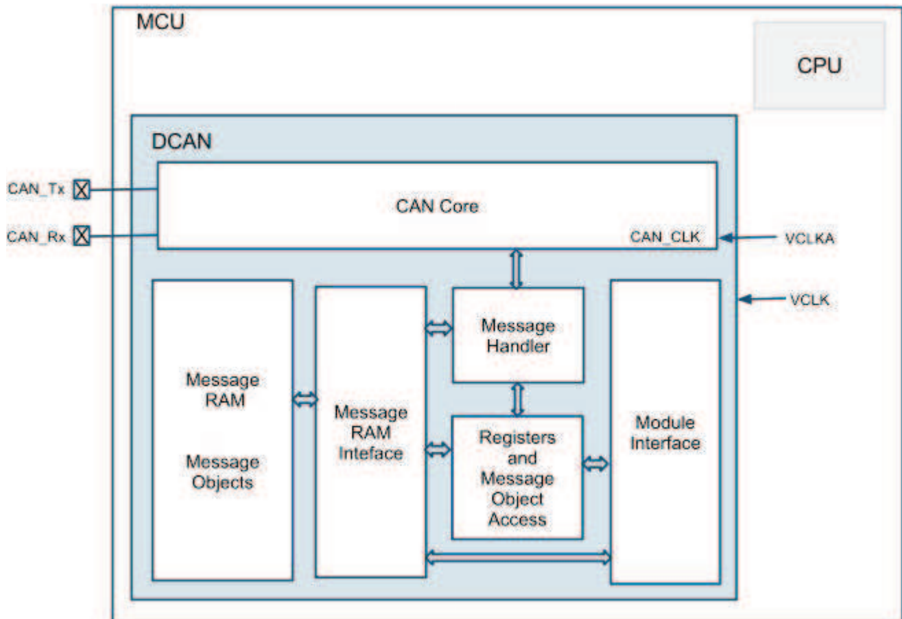
Figure 24-1. Block Diagram
