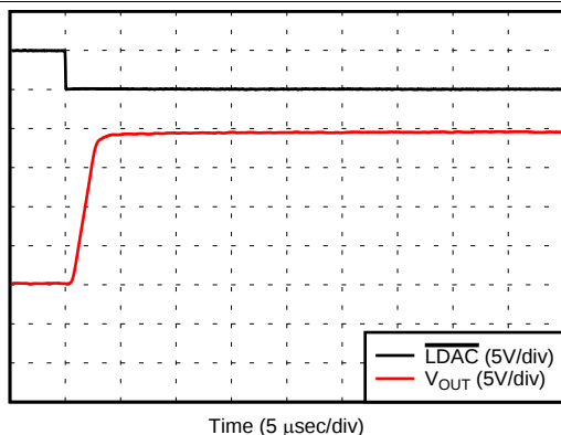
Time (5 \mu\text{sec/div} )
