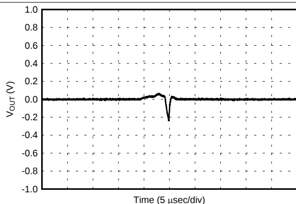
Time (5 \mu\text{sec/div} )
