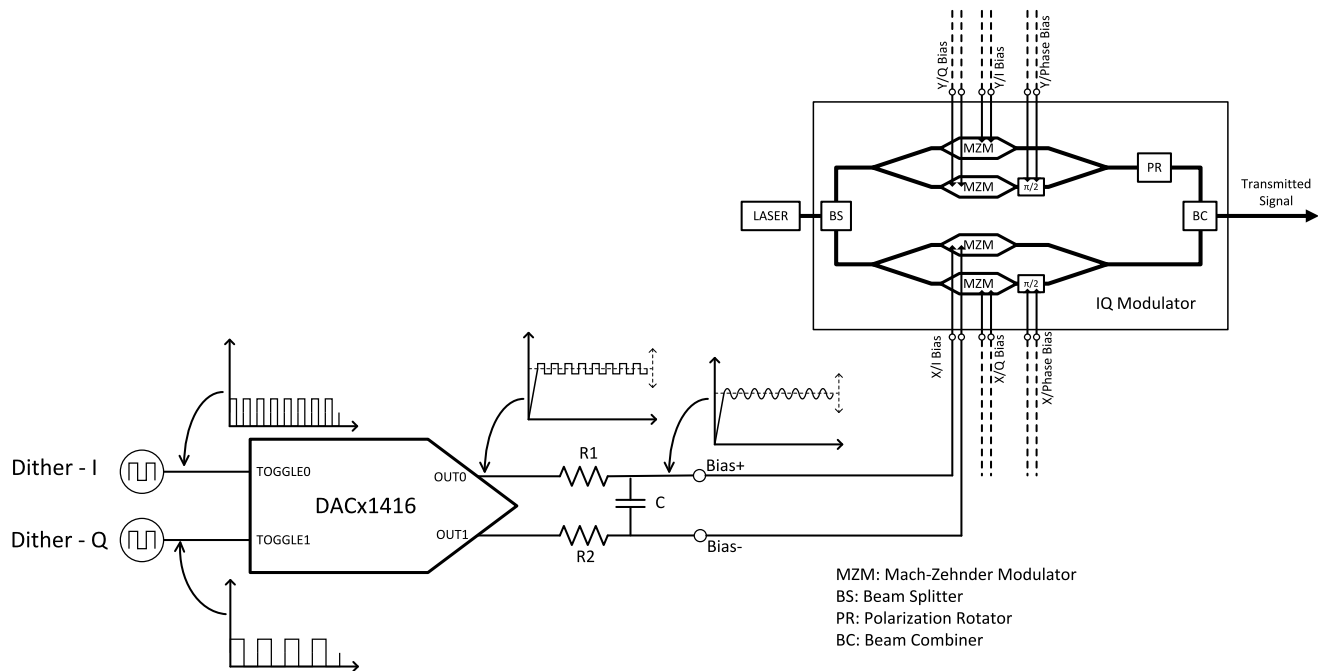
Figure 67. Biasing a Mach Zehnder Modulator
