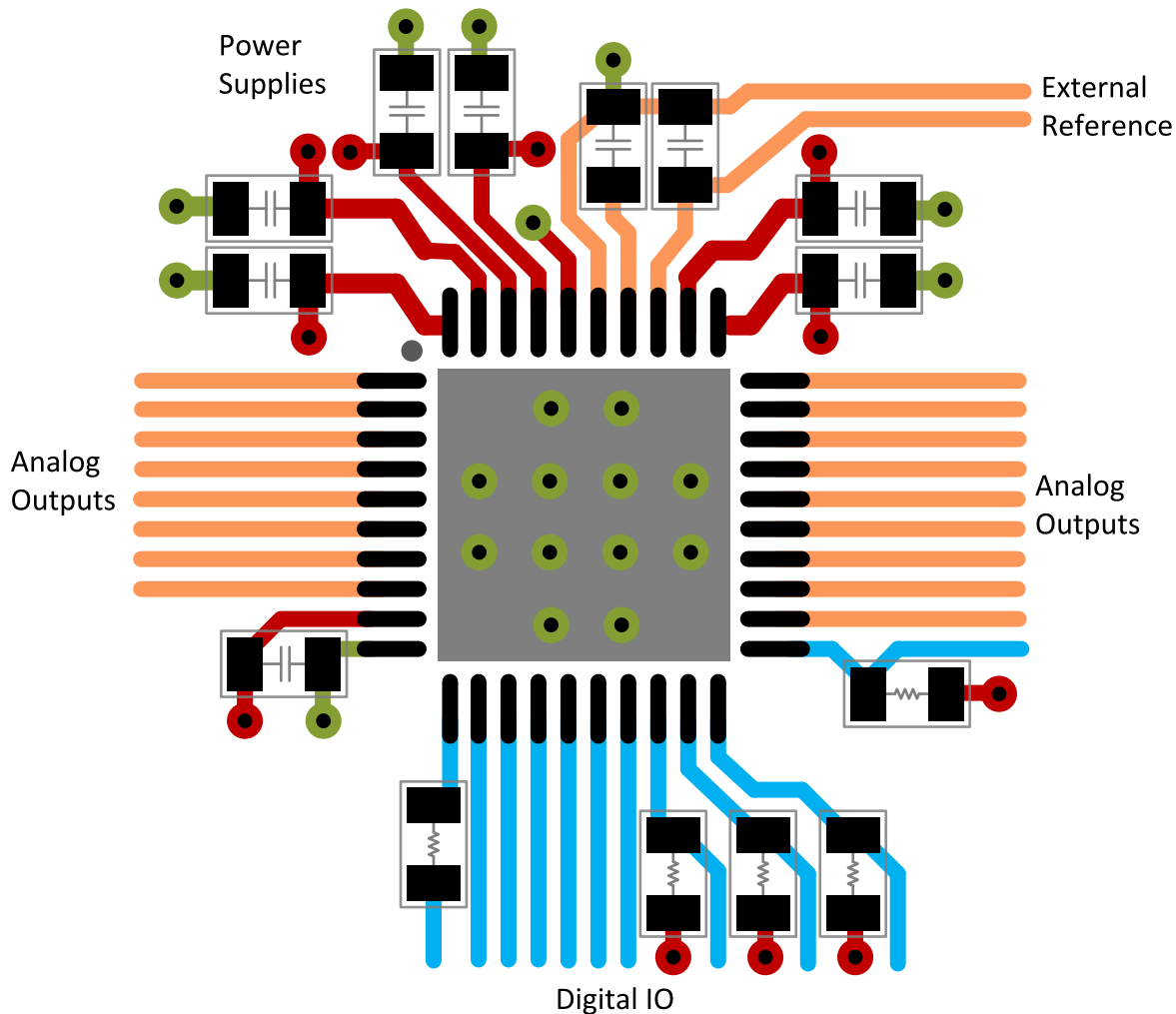
Figure 70. Example Layout
