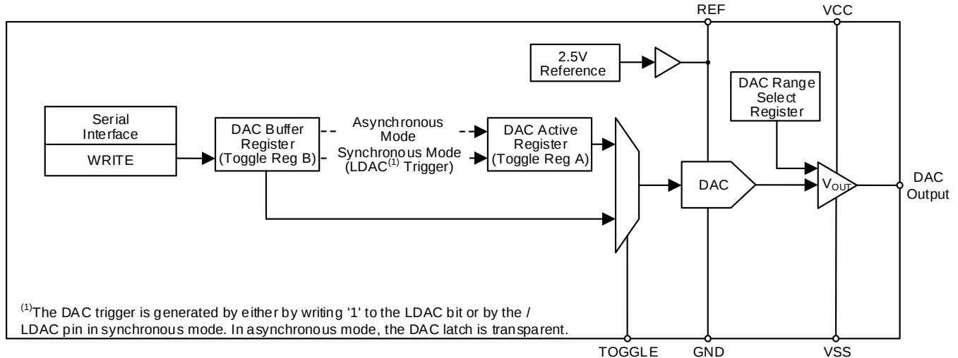
Figure 47. DACx1416 DAC Block Diagram
