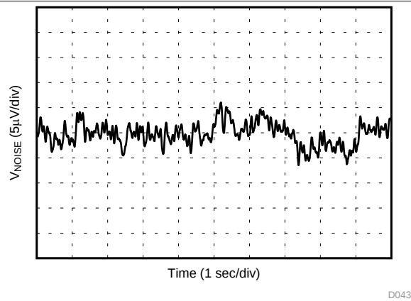
Figure 43. Internal Reference Noise
