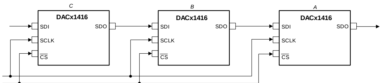
Figure 51. Daisy-Chain Layout
