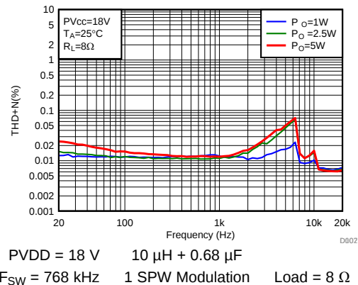
Figure 117. THD+N vs Frequency
