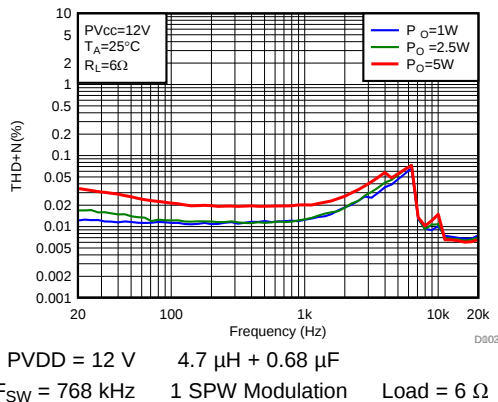
Figure 116. THD+N vs Frequency
