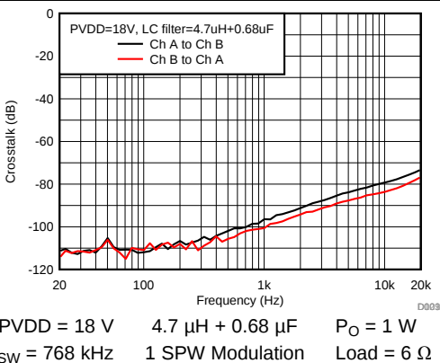
Figure 27. Crosstalk
