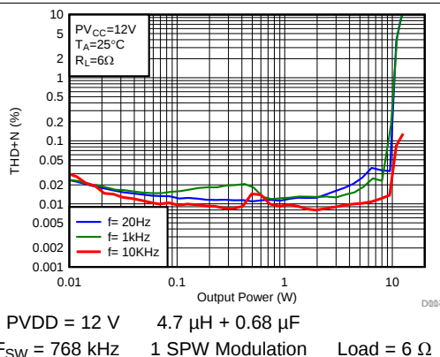
Figure 118. THD+N vs Output Power
