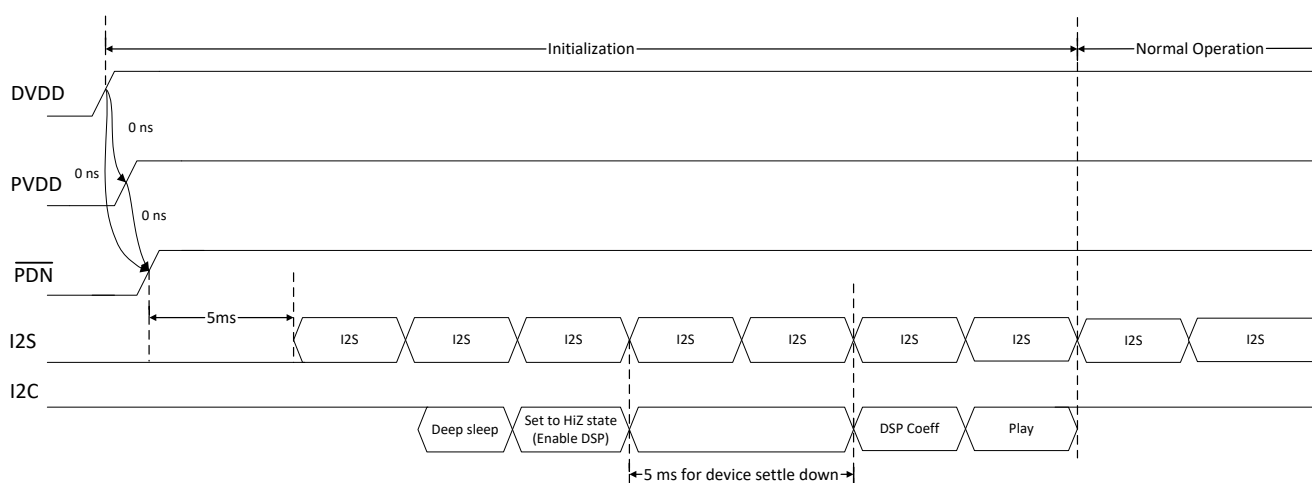
Figure 68. Start-up Sequence
