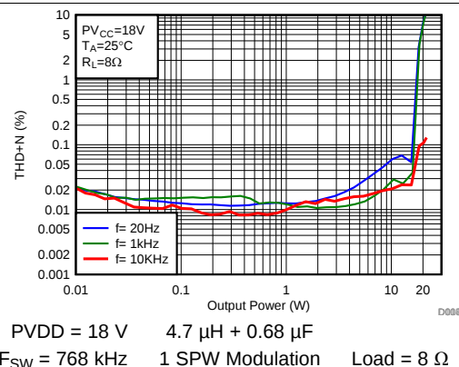
Figure 119. THD+N vs Output Power
