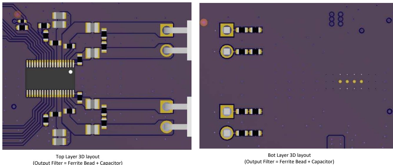
Figure 124. 2.0 (Stereo BTL with Ferrite bead as the output filter) 3-D View
