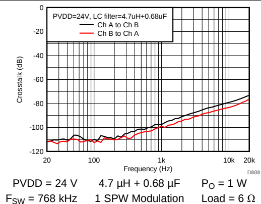
Figure 28. Crosstalk
