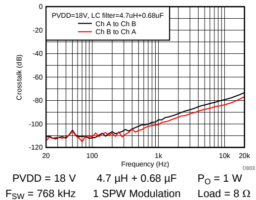
Figure 30. Crosstalk
