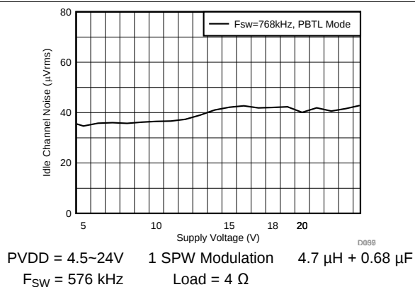
Figure 51. Idle Channel Noise vs Supply Voltage
