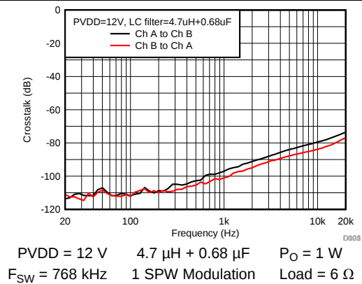
Figure 26. Crosstalk
