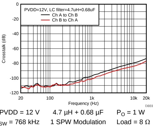
Figure 29. Crosstalk
