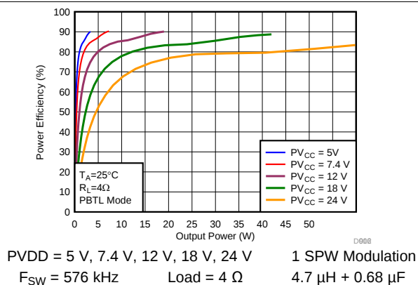
Figure 52. Efficiency vs Output Power
