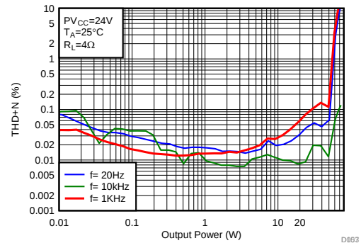
Figure 122. THD+N vs Output Power
