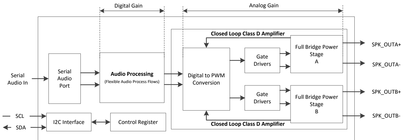
Figure 61. Speaker Amplifier Gain
