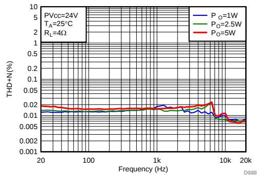
Figure 121. THD+N vs Frequency
