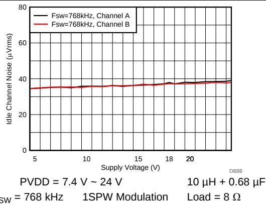
Figure 25. Idle Channel Noise vs Supply Voltage
