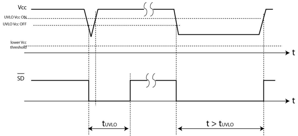
Figure 5. UVLO timing (without contribution of the RC network on \overline{\text{SD}} )
