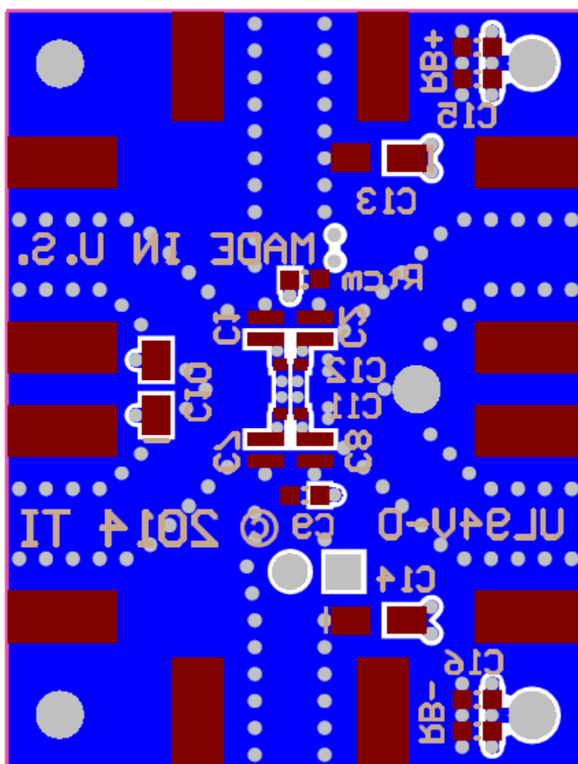
Figure 7. Bottom Layer
