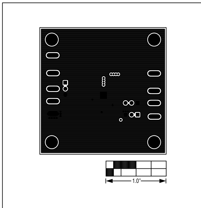
Figure 14. MAX17503 5V Output EV Kit PCB Layout—Inner Layer 1
