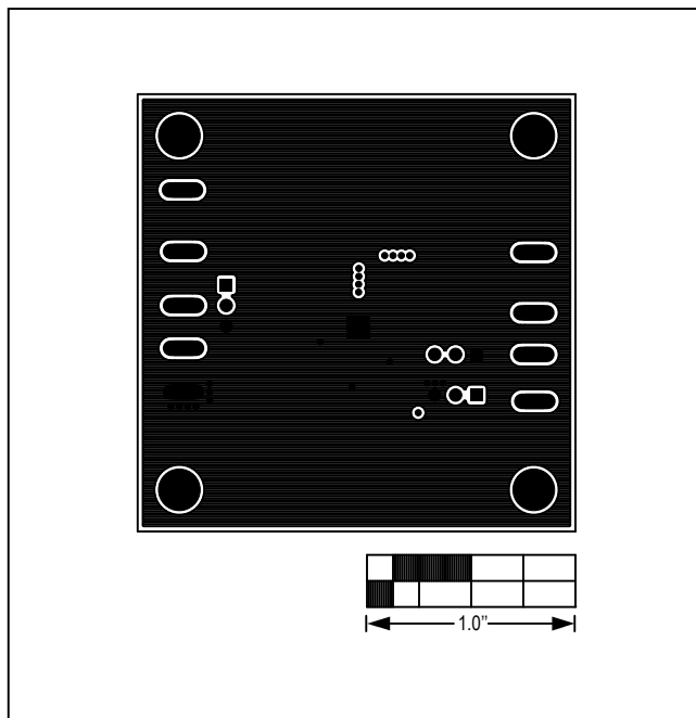
Figure 15. MAX17503 5V Output EV Kit PCB Layout—Inner Layer 2
