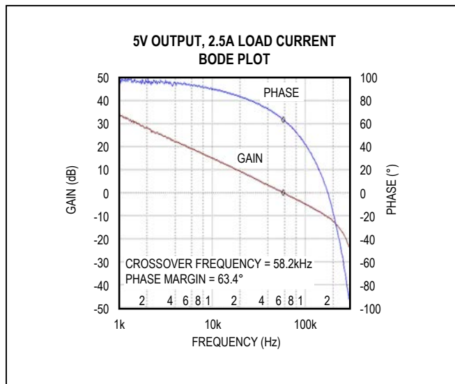
Figure 6. MAX17503 5V Output Full Load Bode Plot ( V_{IN} = 24V )
