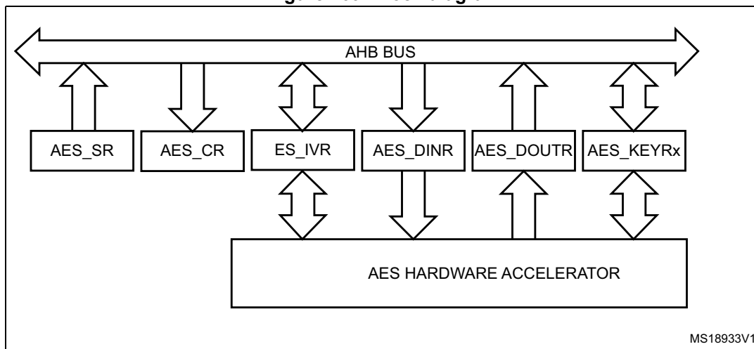
Figure 169. Block diagram
