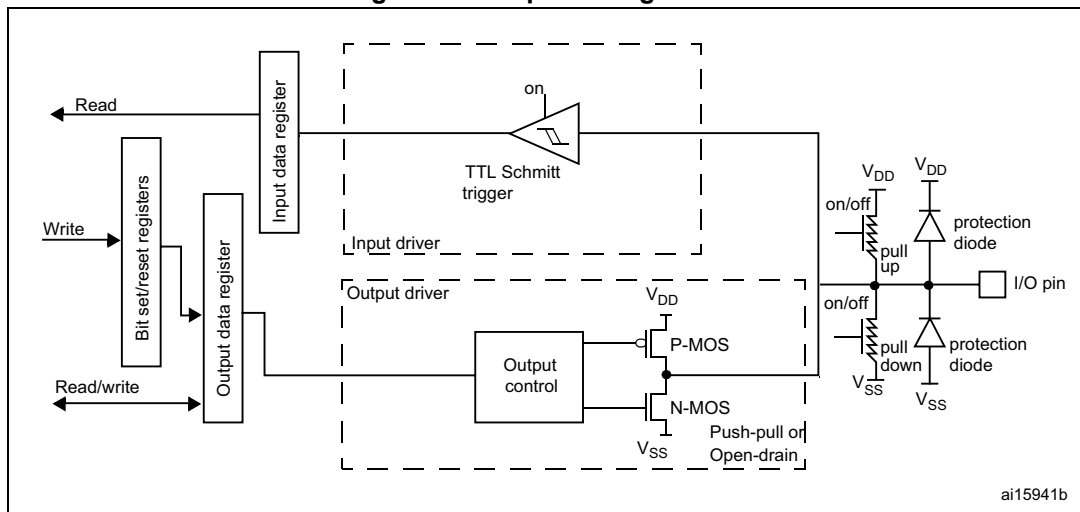
Figure 22. Output configuration
