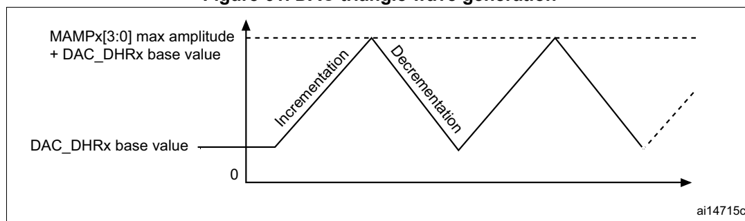
Figure 61. DAC triangle wave generation
