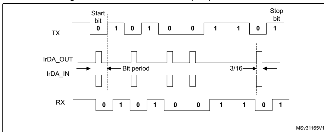
Figure 233. IrDA data modulation (3/16) -Normal mode
