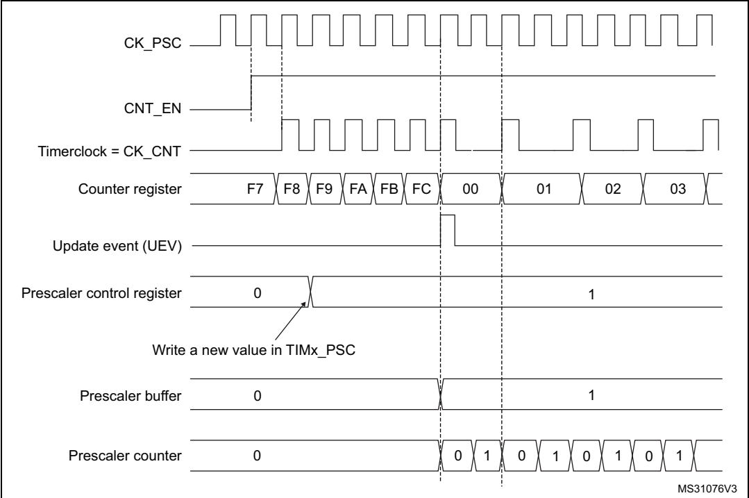
Figure 155. Counter timing diagram with prescaler division change from 1 to 2
