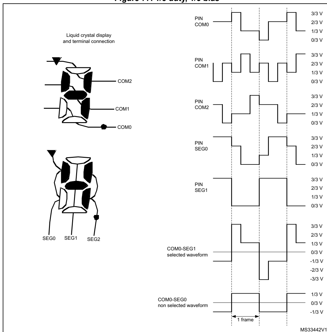
Figure 77. 1/3 duty, 1/3 bias
