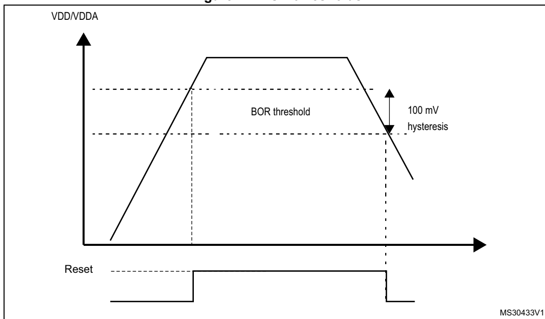
Figure 12. BOR thresholds
