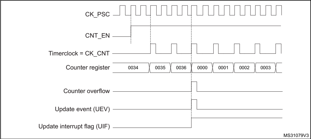
Figure 136. Counter timing diagram, internal clock divided by 2
