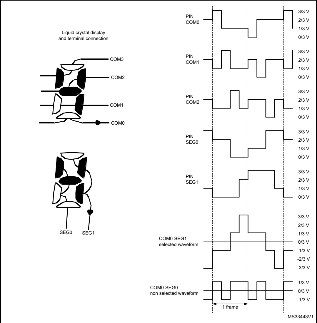
Figure 78. 1/4 duty, 1/3 bias
