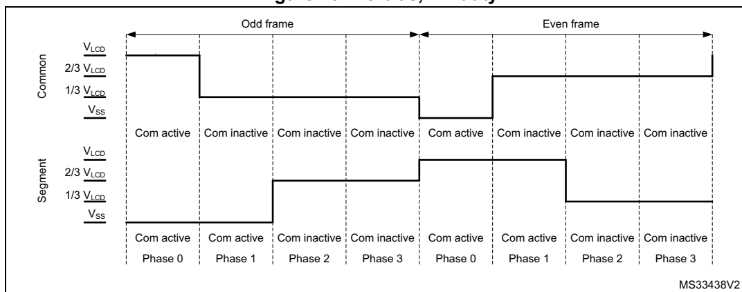
Figure 73. 1/3 bias, 1/4 duty
