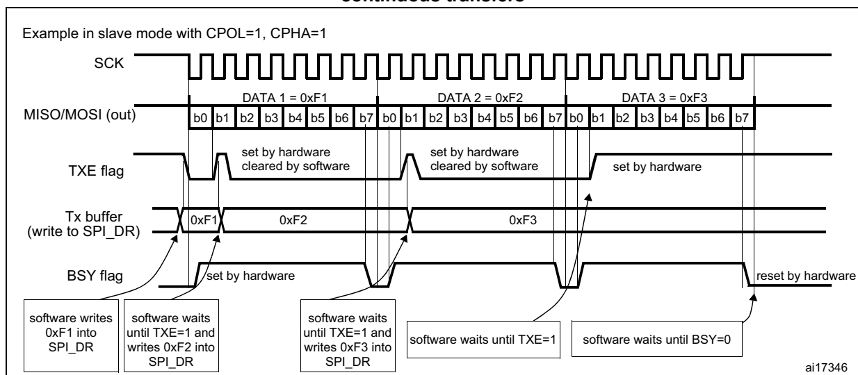
Figure 250. TXE/BSY in Slave transmit-only mode (BIDIMODE=0 and RXONLY=0) in case of continuous transfers
