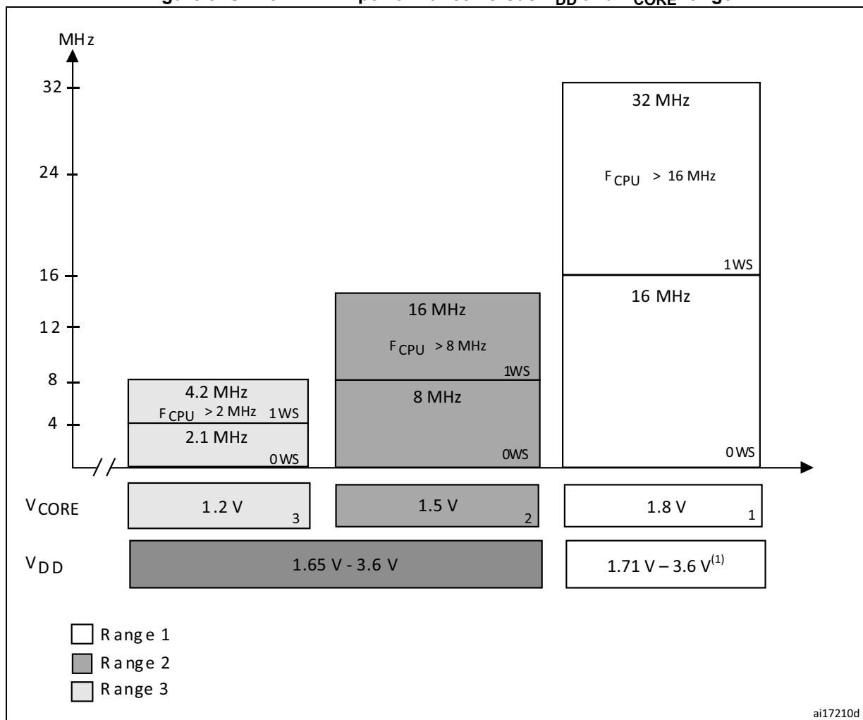
Figure 9. STM32L1xxxx performance versus V_{DD} and V_{CORE} range
