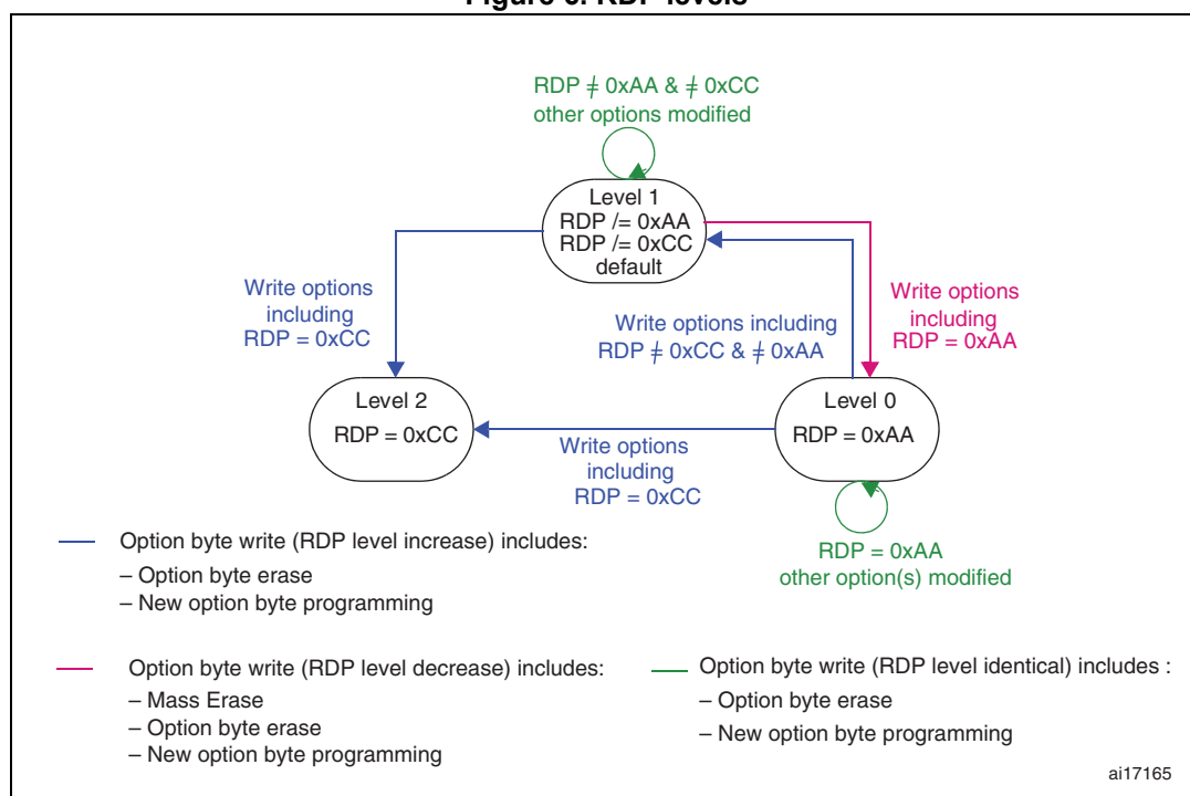
Figure 6. RDP levels
