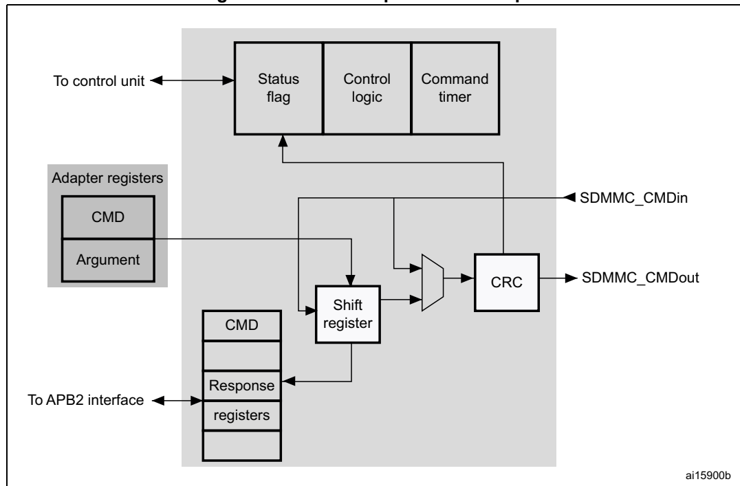
Figure 284. SDIO adapter command path
