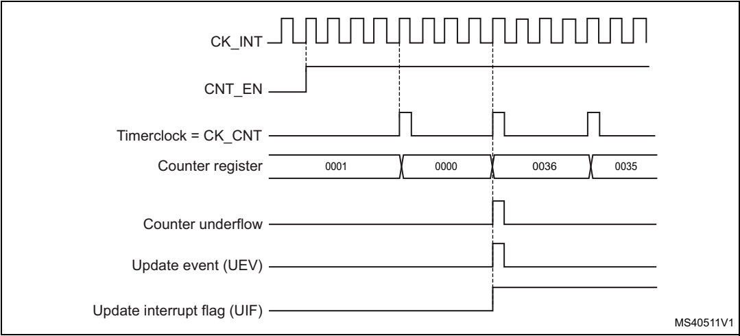
Figure 95. Counter timing diagram, internal clock divided by 4
