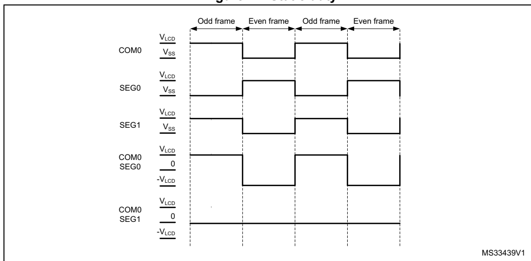
Figure 74. Static duty
