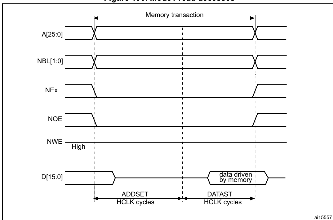
Figure 190. Mode1 read accesses
