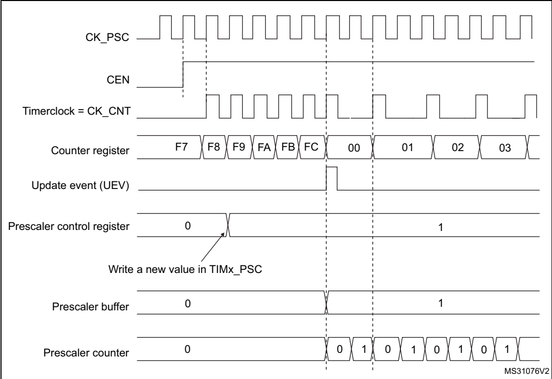
Figure 133. Counter timing diagram with prescaler division change from 1 to 2
