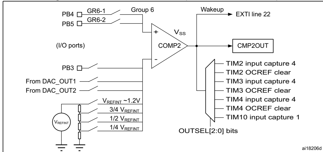
Figure 65. COMP2 interconnections (Cat.1 and Cat.2 devices)
