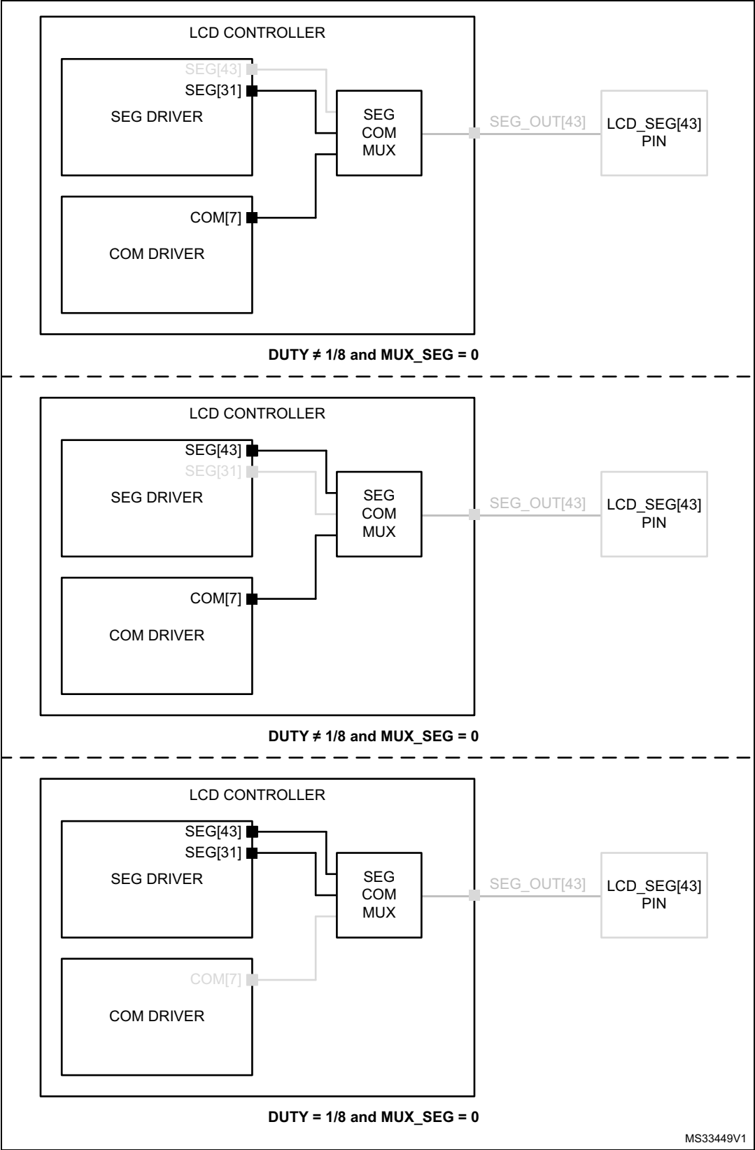
Figure 82. SEG/COM mux feature example
