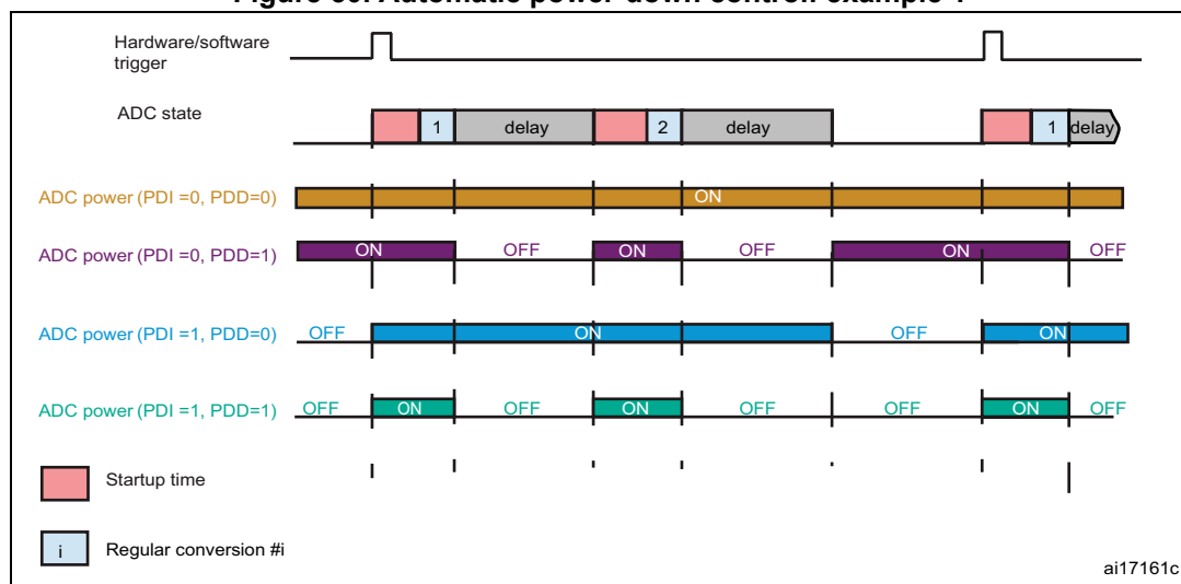
Figure 50. Automatic power-down control: example 1
