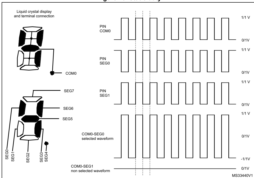
Figure 75. Static duty
