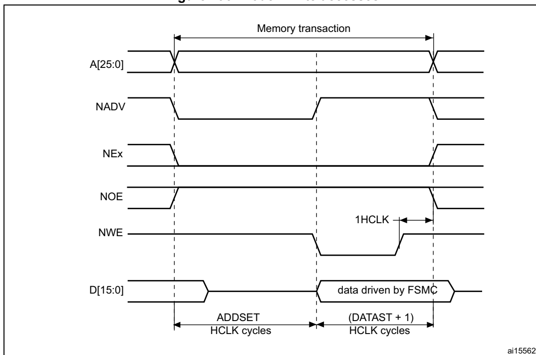
Figure 196. Mode B write accesses
