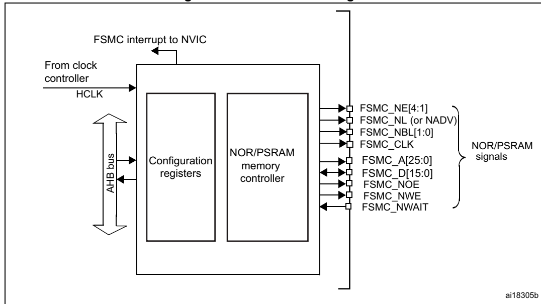
Figure 188. FSMC block diagram
