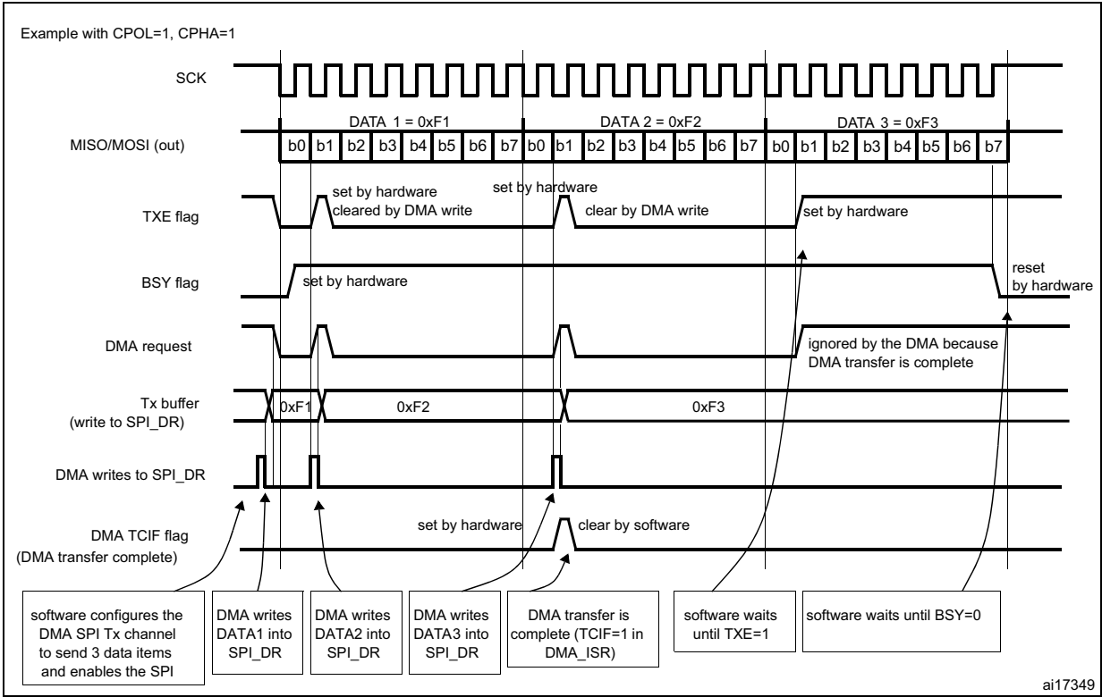
Figure 253. Transmission using DMA
