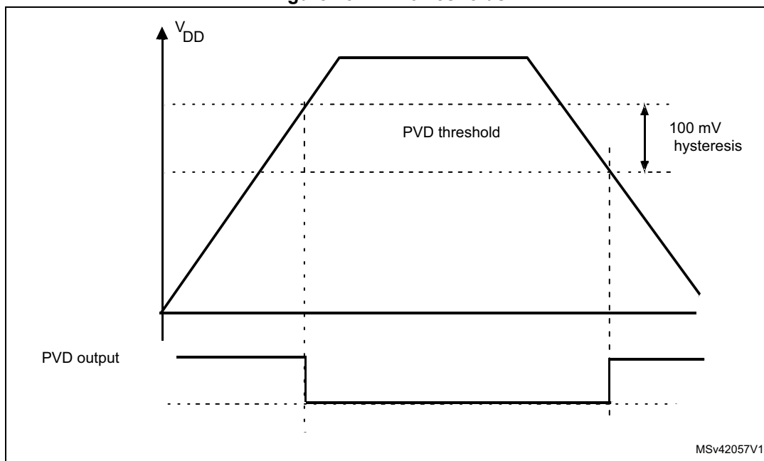
Figure 13. PVD thresholds
