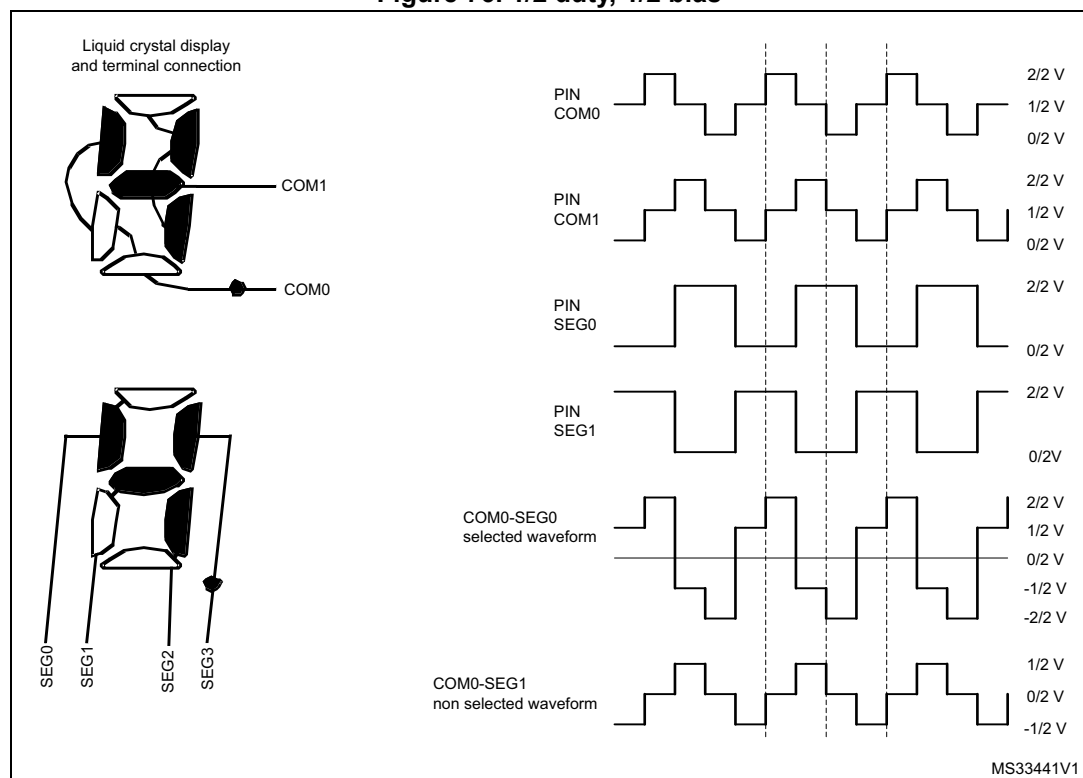
Figure 76. 1/2 duty, 1/2 bias
