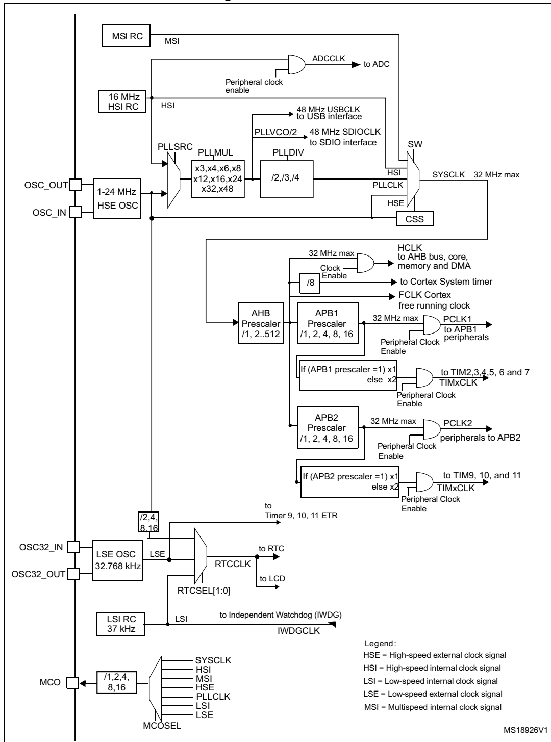
Figure 15. Clock tree
