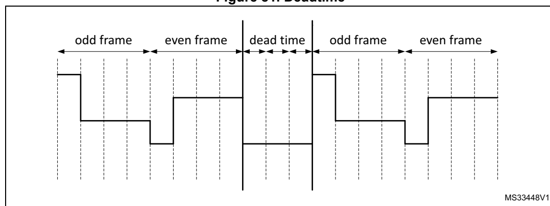
Figure 81. Deadtime
