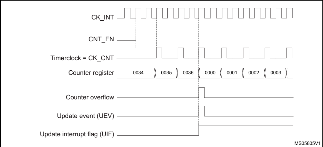
Figure 158. Counter timing diagram, internal clock divided by 2
