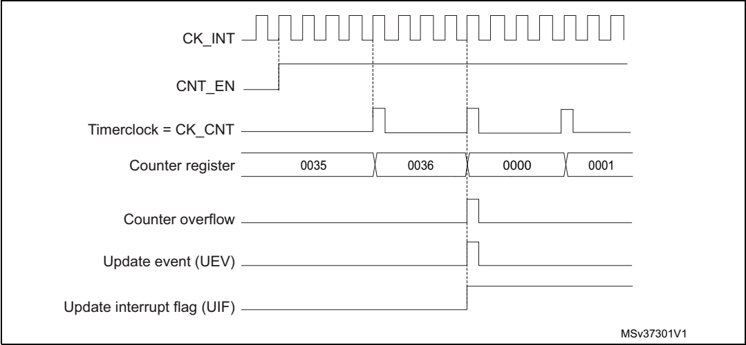
Figure 89. Counter timing diagram, internal clock divided by 4
