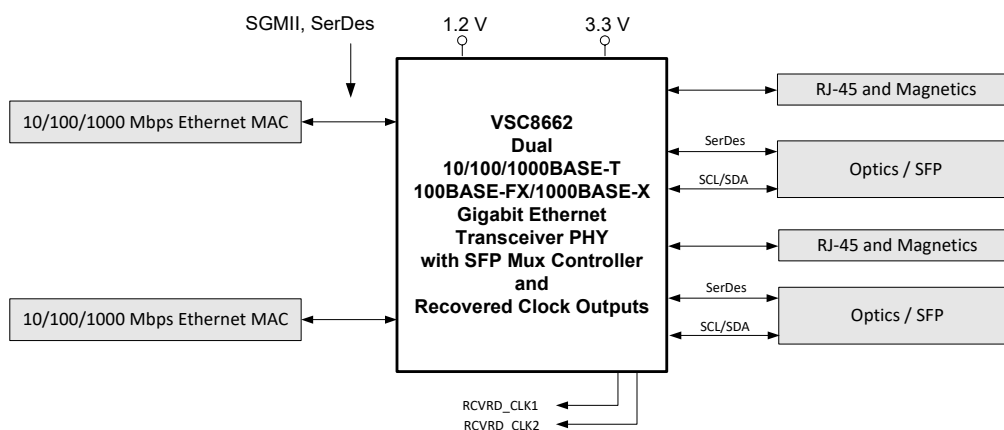
Figure 1 • Typical Application
