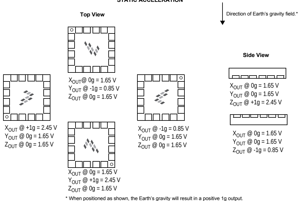
Figure 18. Orientation and Output Values for MMA7260QT, MMA6270QT and MMA6280QT
