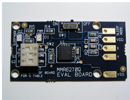
Figure 5. Photo of MMA6270QT Evaluation Board (similar to MMA6271QT Evaluation Board)
