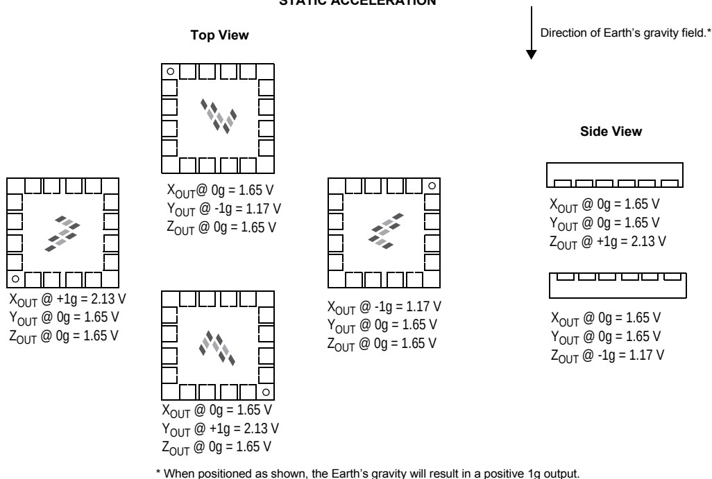
Figure 19. Orientation and Output Values for MMA7261QT
