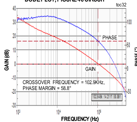
MAX17503S, 5V OUTPUT, 2.5A LOAD CURRENT, BODE PLOT, FIGURE 4c CIRCUIT
