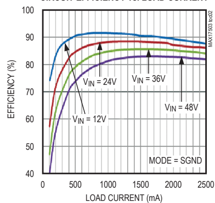
MAX17503, 3.3V OUTPUT, PWM MODE, FIGURE 4b CIRCUIT EFFICIENCY vs. LOAD CURRENT
