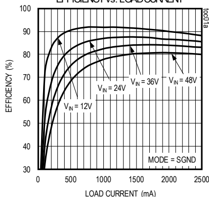
MAX17503S, 5V OUTPUT, PWM MODE, FIGURE 4c CIRCUIT, EFFICIENCY vs. LOAD CURRENT
