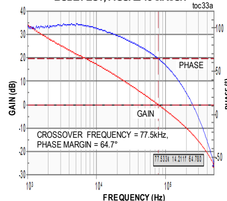
MAX17503S, 3.3V OUTPUT, 2.5A LOAD CURRENT, BODE PLOT, FIGURE 4c CIRCUIT
