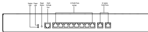
Figure 1: PDS208 Front Panel
