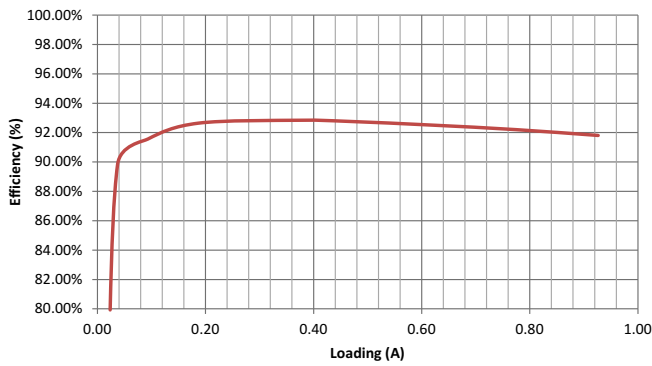
Figure 3. Efficiency ( V_{IN} = 12\text{ V} , V_{LNB} = 18.6\text{ V} )
