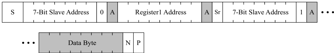
Figure 55. I 2 C Read Data Format
