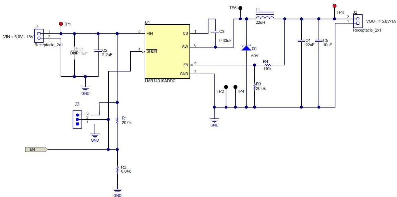
Figure 3. LMR14010AEVM Schematic
