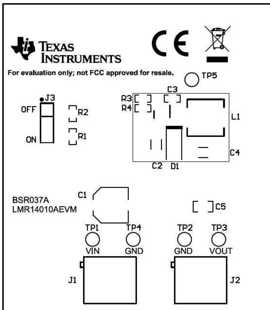
Figure 4. Top Assembly
