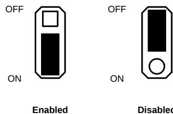
Figure 2. Enable Jumper Setting
