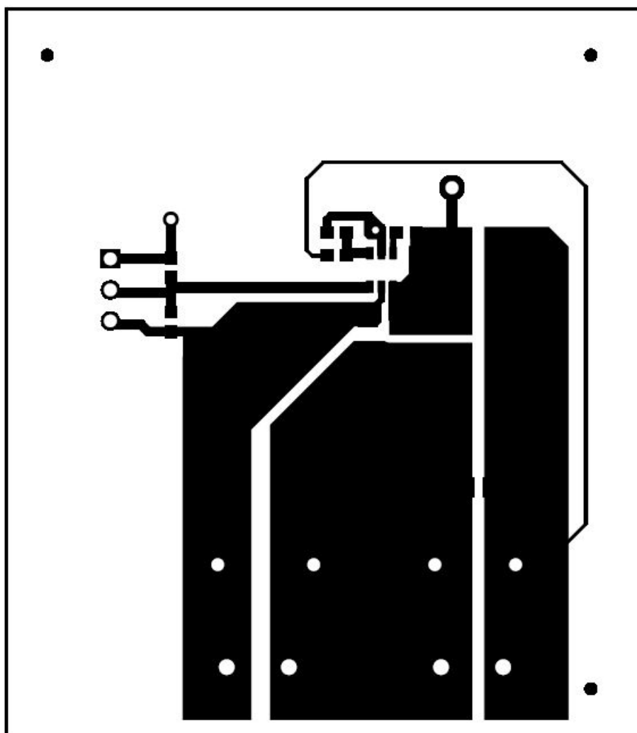
Figure 5. Top Layer
