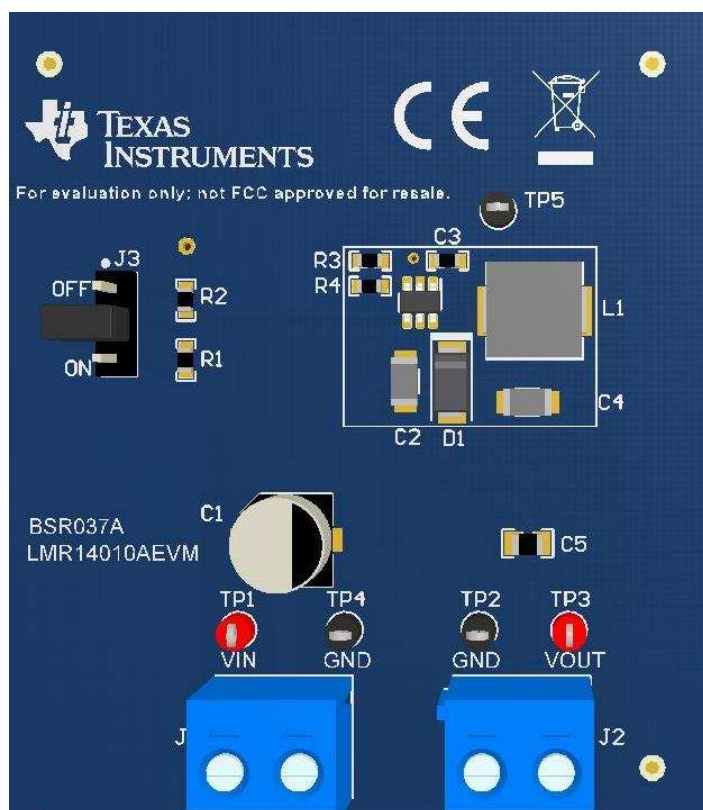
Figure 1. LMR14010AEVM Board
