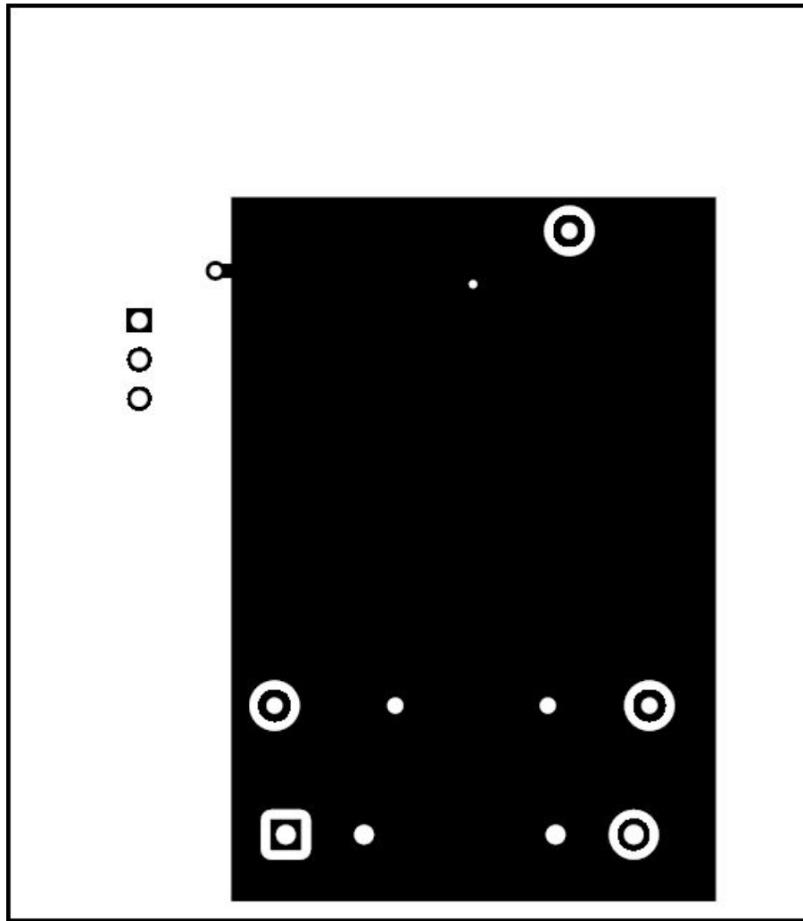
Figure 6. Bottom Layer
