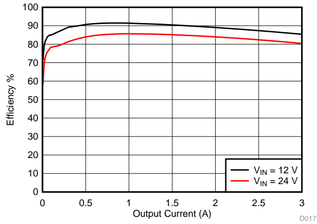
Figure 1. TPS54334EVM-722 Efficiency
