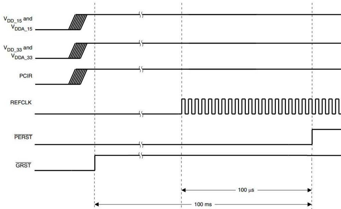
Figure 4. Power-Up Sequence
