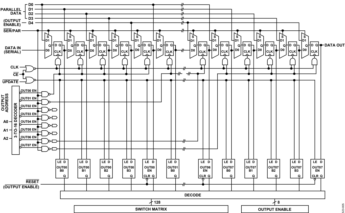
Figure 5. Logic Diagram
