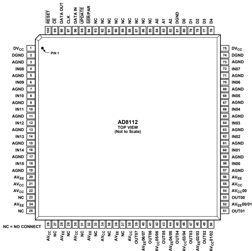
Figure 6. Pin Configuration
