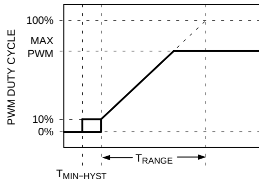
Figure 60. Changing \text{PWM}_{\text{MAX}} Does Not Change the AFC Slope
