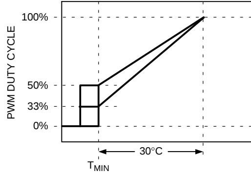
Figure 58. Adjusting \text{PWM}_{\text{MIN}} Changes the Automatic Fan Control Slope
