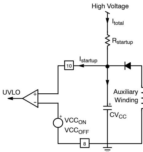
Figure 3. The Startup Resistor Brings V_{\text{CC}} Above 15 V
