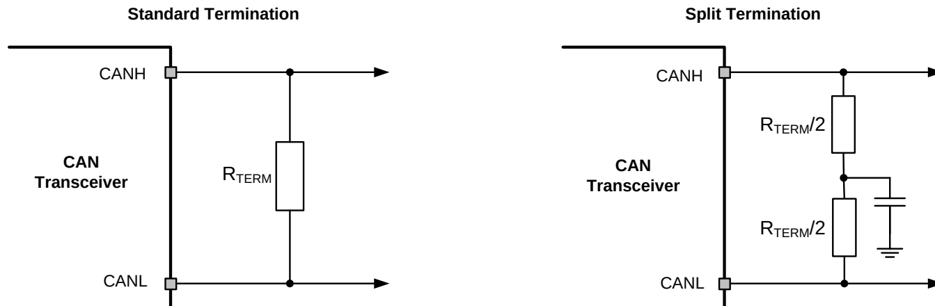
Figure 28. CAN Termination
