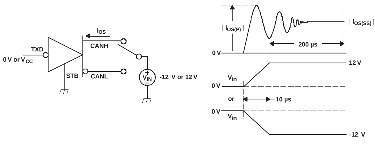
Figure 21. Driver Short-Circuit Current Test and Waveforms
