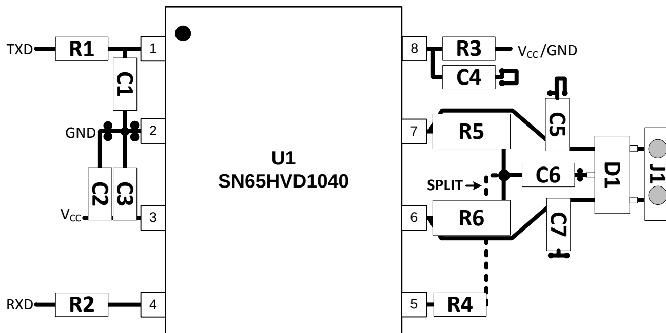
Figure 33. Layout Recommendation
