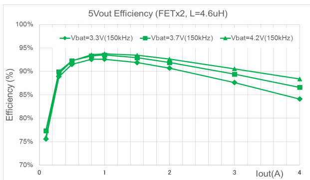
Figure 25. Boost Efficiency (VOUT = 5 V)
