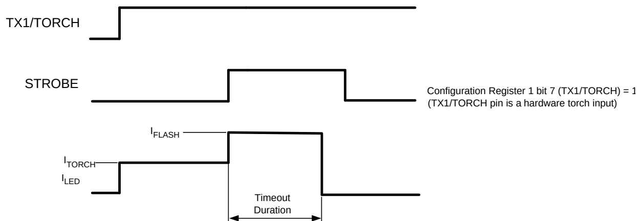
Figure 37. TX1/Torch Configured as a Hardware Torch Input
