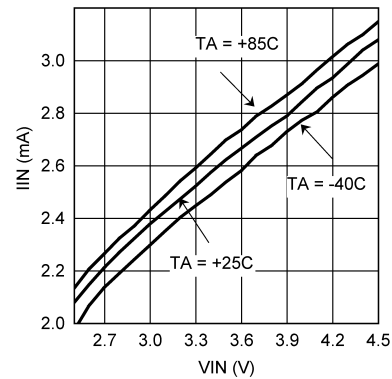
Figure 15. Active (Switching) Supply Current vs V_{IN}
