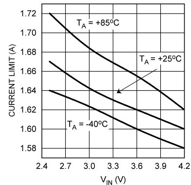
Figure 17. Closed Loop Current Limit vs V_{IN} (Flash Duration Register Bits [6:5] = 01) (1)
