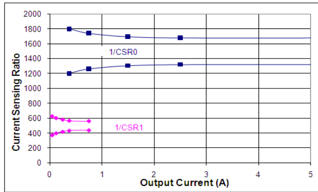
Figure 19. Current sensing ratio versus output current
