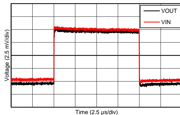
Figure 28. Positive Overload Recovery
