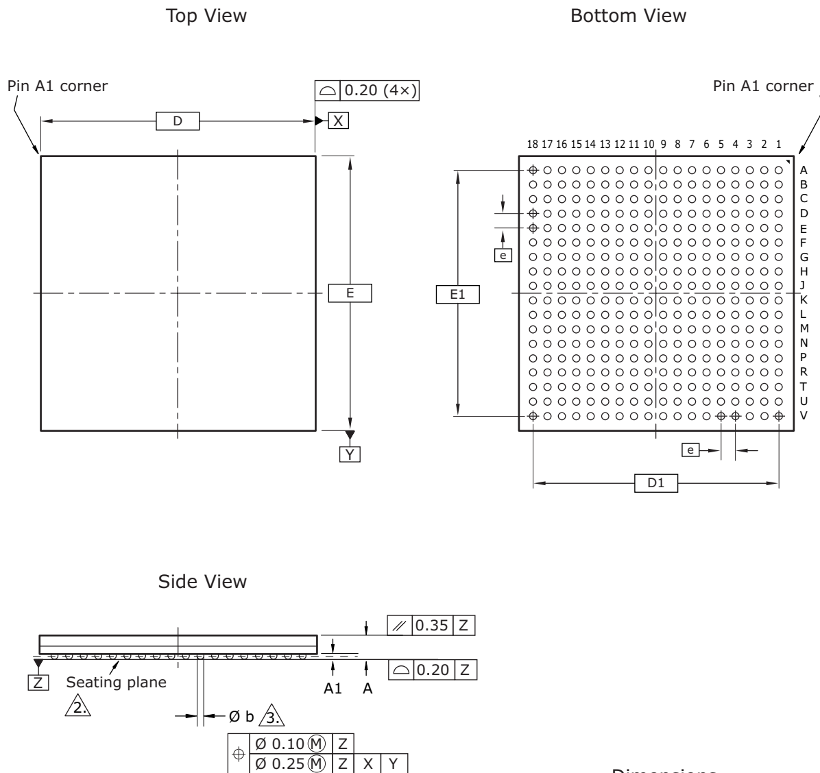
Figure 152 • Package Drawing
