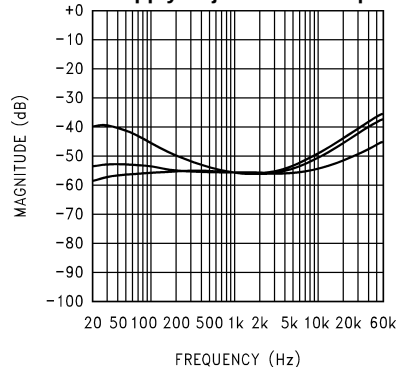
Figure 28. V_{DD} = 12\text{V} , R_L = 8\Omega , SE operation, V_{\text{RIIPPLE}} = 200\text{mV}_{\text{p-p}} , A_V = 10 , at (from top to bottom at 60Hz): C_{\text{BYPASS}} = 1\mu\text{F} , C_{\text{BYPASS}} = 4.7\mu\text{F} , C_{\text{BYPASS}} = 10\mu\text{F}
