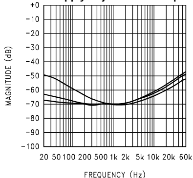
Figure 25. V_{DD} = 12\text{V} , R_L = 8\Omega , BTL operation, V_{\text{RIIPPLE}} = 200\text{mV}_{\text{p-p}} , at (from top to bottom at 60Hz): C_{\text{BYPASS}} = 1\mu\text{F} , C_{\text{BYPASS}} = 4.7\mu\text{F} , C_{\text{BYPASS}} = 10\mu\text{F}
