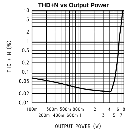
Figure 14. V_{DD} = 12V , R_L = 8\Omega , BTL operation, f_{IN} = 1kHz
