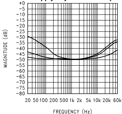
Figure 27. V_{DD} = 12\text{V} , R_L = 8\Omega , BTL operation, V_{\text{RIIPPLE}} = 200\text{mV}_{\text{p-p}} , A_V = 20 , at (from top to bottom at 60Hz): C_{\text{BYPASS}} = 1\mu\text{F} , C_{\text{BYPASS}} = 4.7\mu\text{F} , C_{\text{BYPASS}} = 10\mu\text{F}
