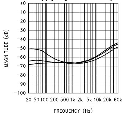
Figure 26. V_{DD} = 12\text{V} , R_L = 8\Omega , SE operation, V_{\text{RIIPPLE}} = 200\text{mV}_{\text{p-p}} , at (from top to bottom at 60Hz): C_{\text{BYPASS}} = 1\mu\text{F} , C_{\text{BYPASS}} = 4.7\mu\text{F} , C_{\text{BYPASS}} = 10\mu\text{F}
