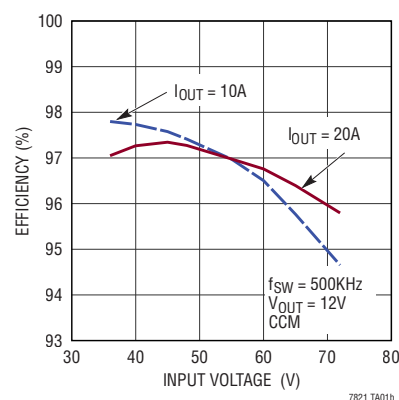
Efficiency at Various V_{IN} for V_{OUT} = 12V
