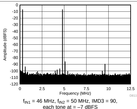
Figure 11. FFT for Two-Tone Input Signal (–7 dBFS at 46 MHz and 50 MHz)
