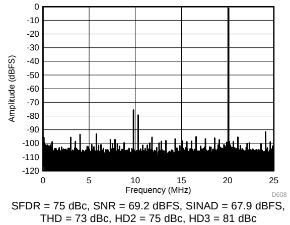
Figure 38. FFT for 270-MHz Input Signal (Dither Off)
