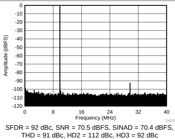
Figure 63. FFT for 70-MHz Input Signal (Dither On)
