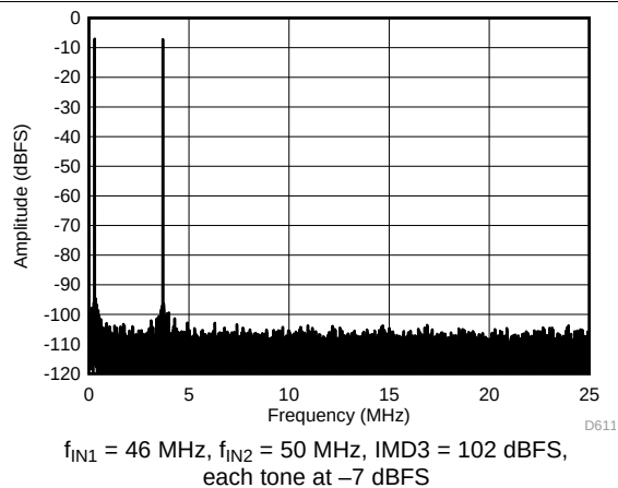
Figure 41. FFT for Two-Tone Input Signal ( -7\text{ dBFS} at 46 MHz and 50 MHz)
