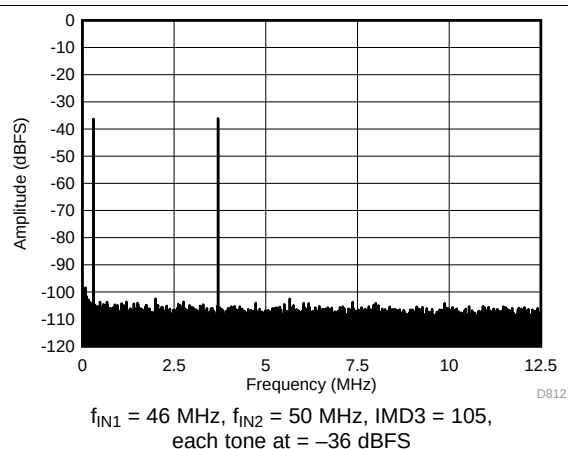
Figure 12. FFT for Two-Tone Input Signal (–36 dBFS at 46 MHz and 50 MHz)
