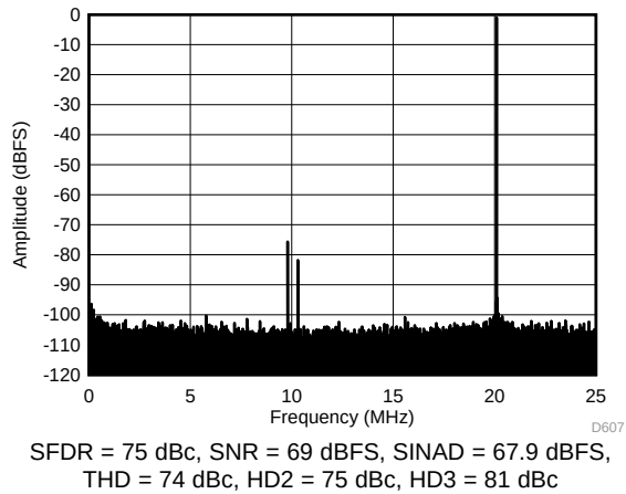
Figure 37. FFT for 270-MHz Input Signal (Dither On)
