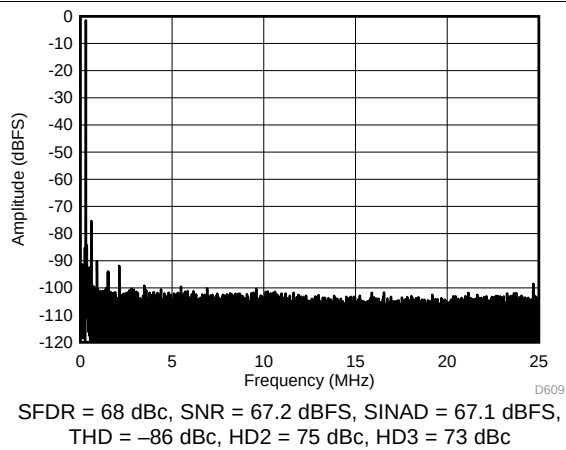
Figure 39. FFT for 450-MHz Input Signal (Dither On)
