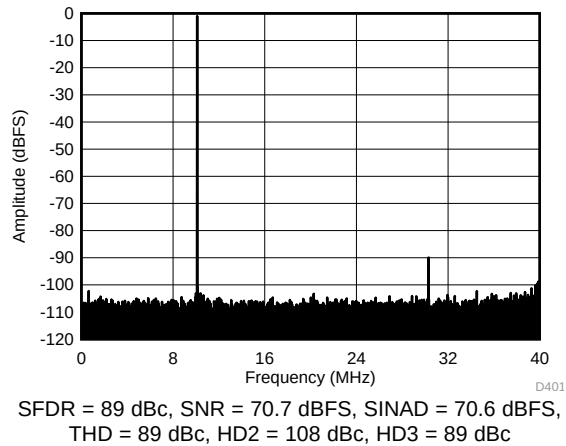
Figure 61. FFT for 10-MHz Input Signal (Dither On)
