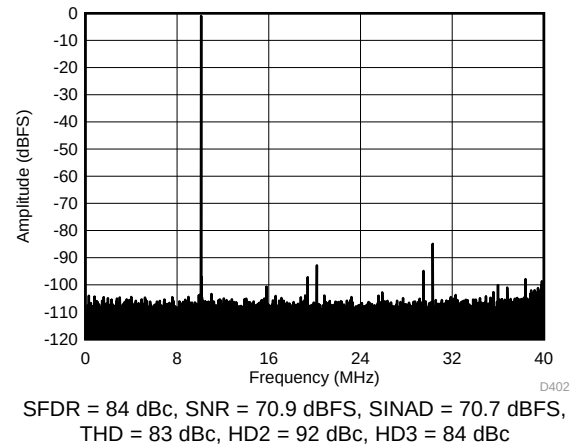
Figure 62. FFT for 10-MHz Input Signal (Dither Off)
