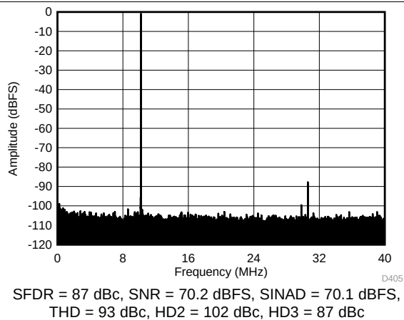
Figure 65. FFT for 170-MHz Input Signal (Dither On)
