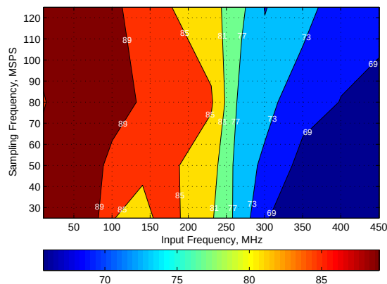
Figure 127. Spurious-Free Dynamic Range (SFDR)
