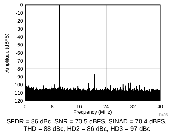
Figure 66. FFT for 170-MHz Input Signal (Dither Off)
