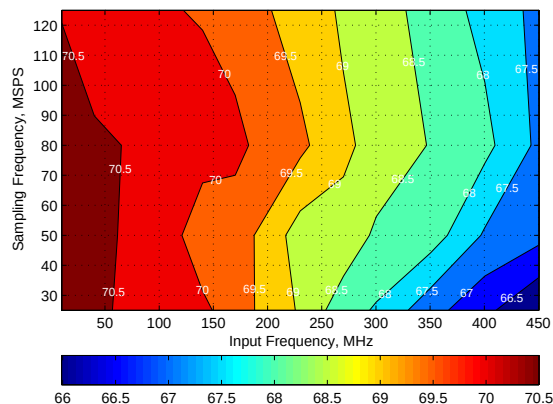
Figure 128. Signal-to-Noise Ratio (SNR)
