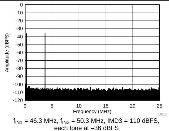
Figure 42. FFT for Two-Tone Input Signal ( -36\text{ dBFS} at 46 MHz and 50 MHz)
