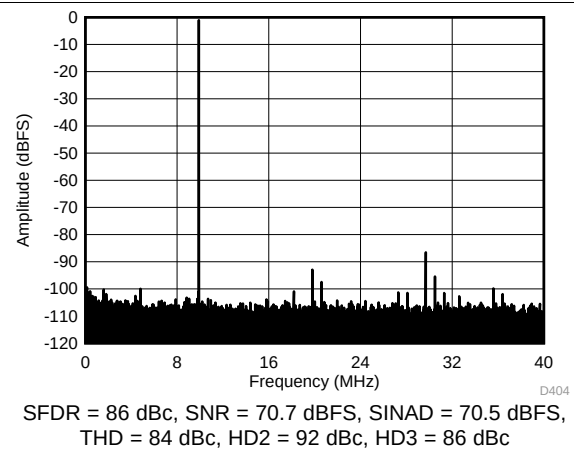
Figure 64. FFT for 70-MHz Input Signal (Dither Off)
