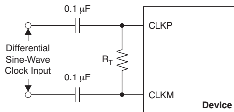
Figure 132. Differential Sine-Wave Clock Driving Circuit
