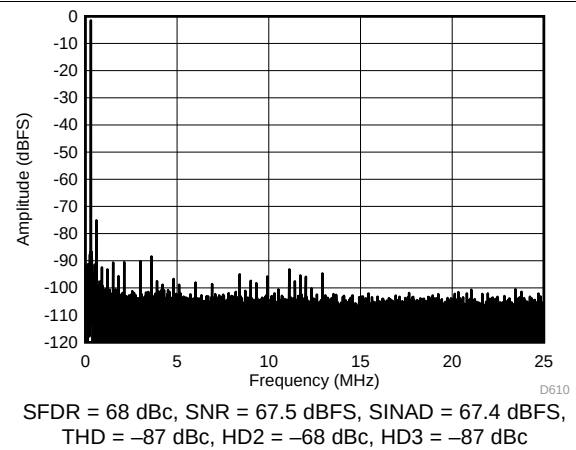
Figure 40. FFT for 450-MHz Input Signal (Dither Off)
