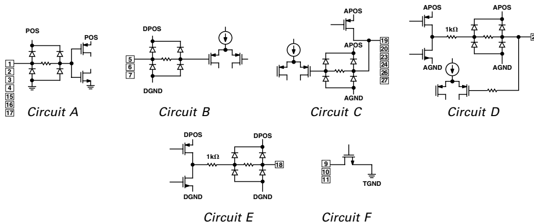
Figure 1. Equivalent Circuits
