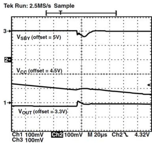
Figure 18. V CC Power Down (V SBY = 5 V, Load = 300 mA)
