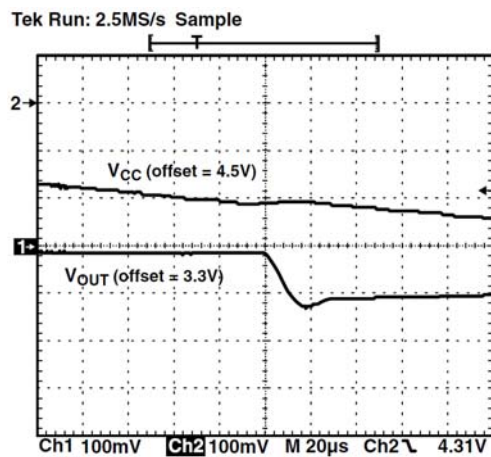
Figure 20. V CC Power Down (V AUX = 3.3 V, Load = 300 mA)
