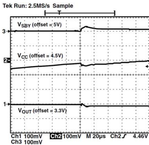
Figure 17. V CC Power Up (V SBY = 5 V, Load = 300 mA)
