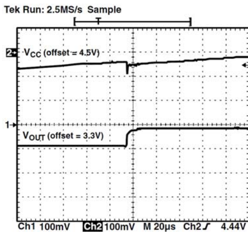
Figure 19. V CC Power Up (V AUX = 3.3 V, Load = 300 mA)
