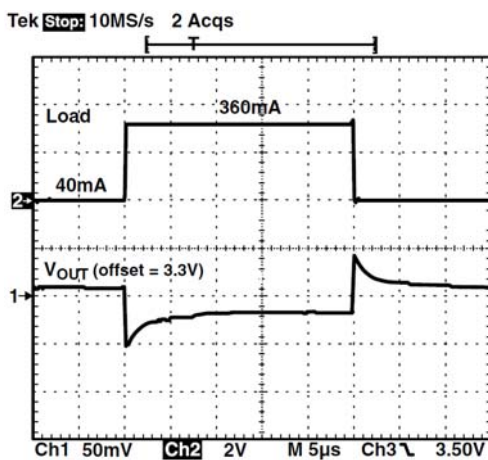
Figure 21. Load Transient Response (10% – 90% Rated)
