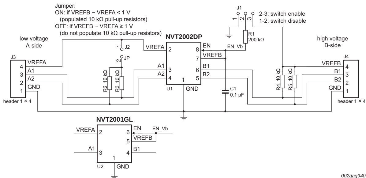
Fig 2. NVT2001GM and NVT2002DP demo board schematic
