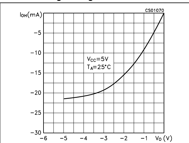
Figure 11. Receiver output current vs output high voltage
