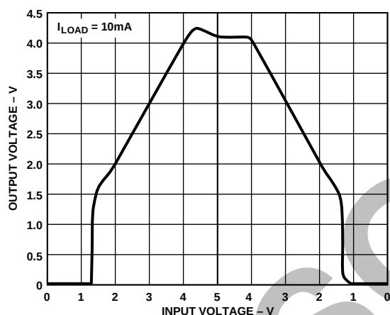
Figure 9. Power-Up/Power-Down*
