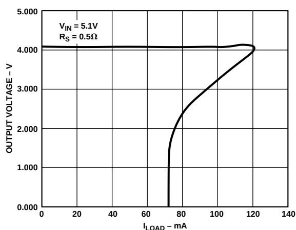
Figure 13. Current Limit Foldback*
