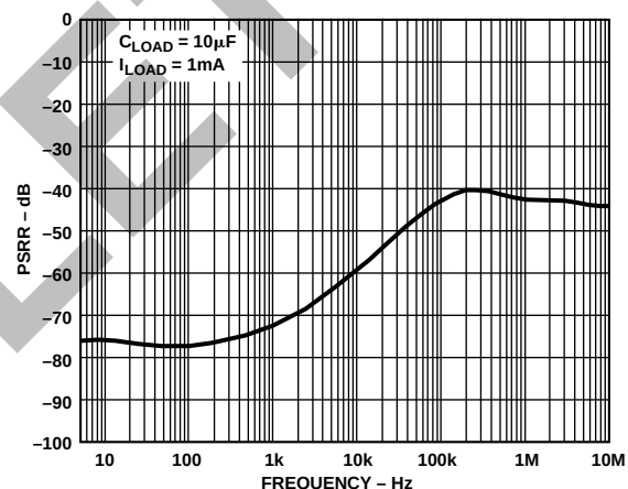
Figure 12. Ripple Rejection*
