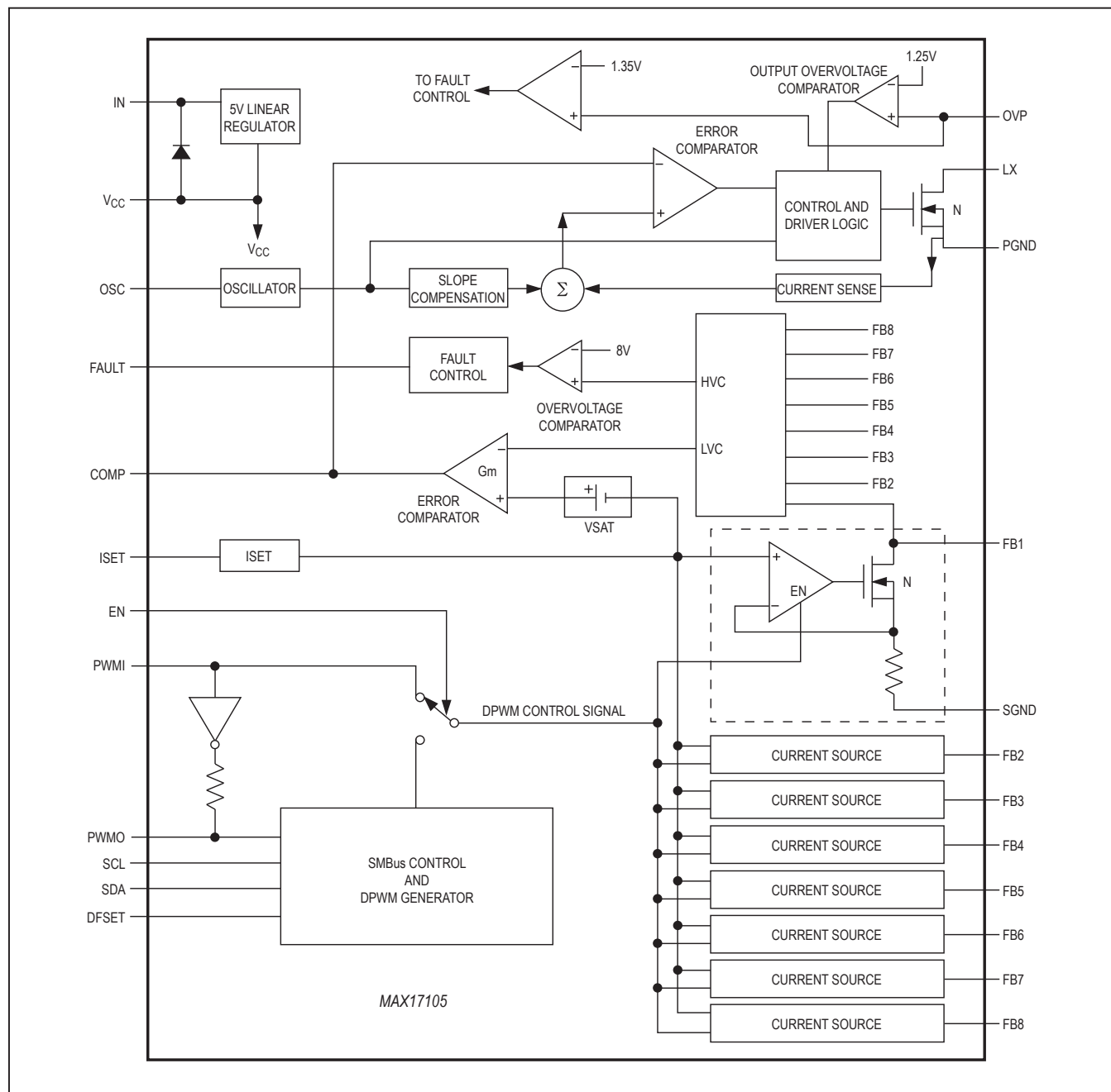
Figure 2. Functional Diagram
