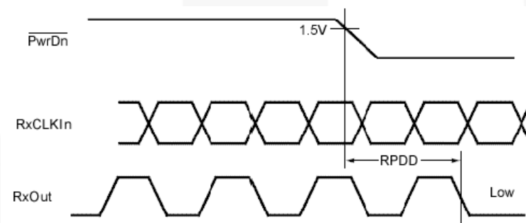
Figure 18. Receiver Power-down Delay
