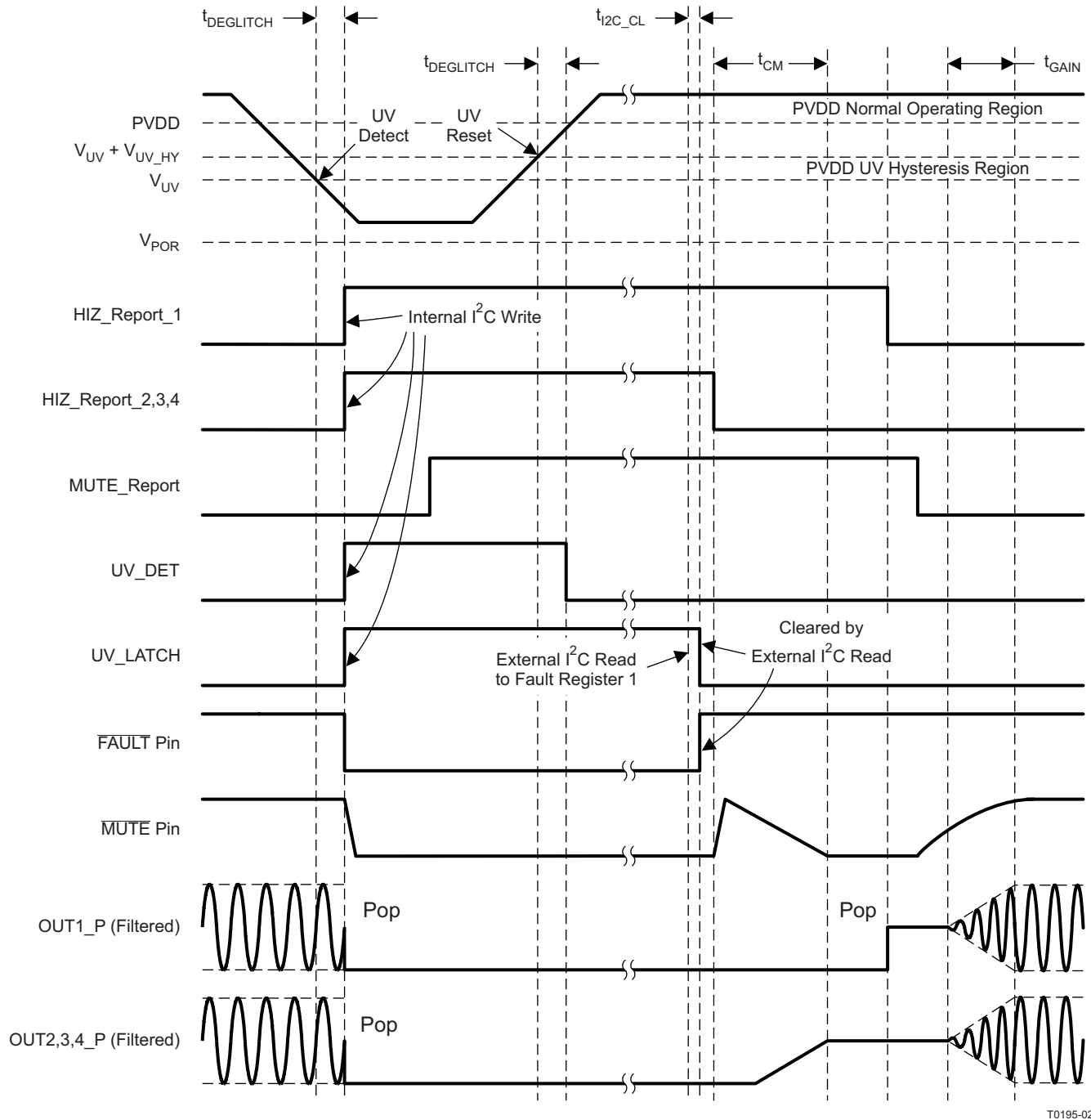
Figure 20. Latched Global-Fault Shutdown and Individual-Channel Restart Timing Diagram (UV Shutdown and Recovery)
