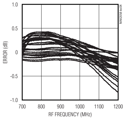
ATTEN B ABS ACCURACY vs. RF FREQUENCY
