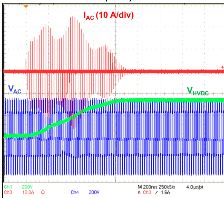
Figure 4: Inrush-current at STEVAL-ISF003V1 start-up on 230 V line (1 mF output DC capacitor)
