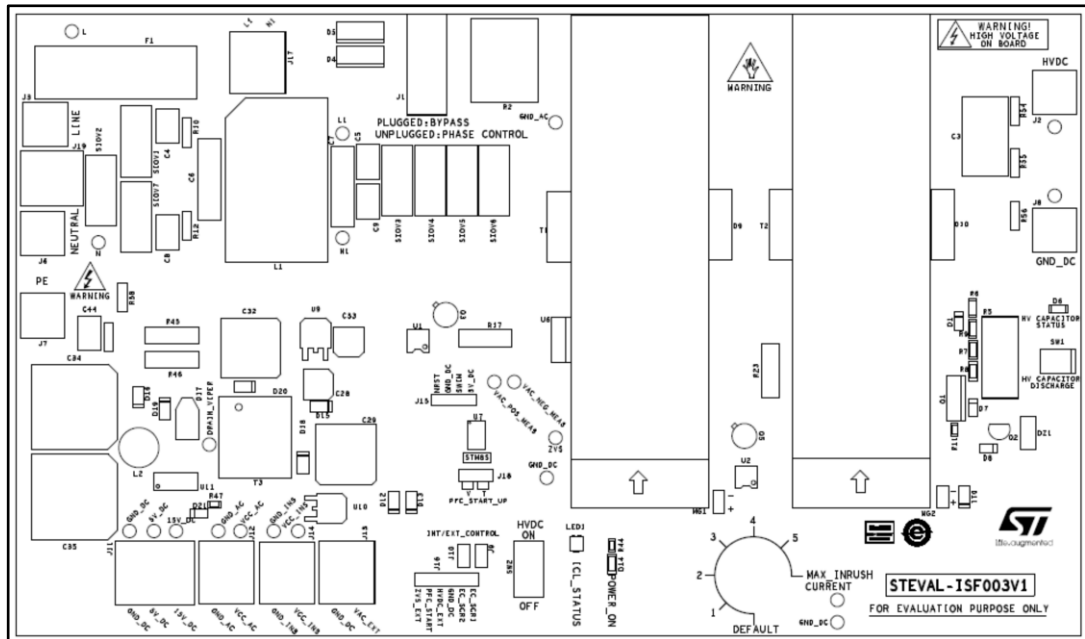
Figure 26: STEVAL-ISF003V1 silk-screen
