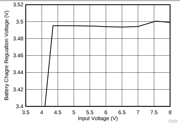
Figure 8. Input Voltage vs Battery Charge Regulation Voltage
