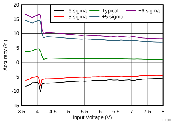
Figure 7. Charge Current Accuracy vs Input Voltage
