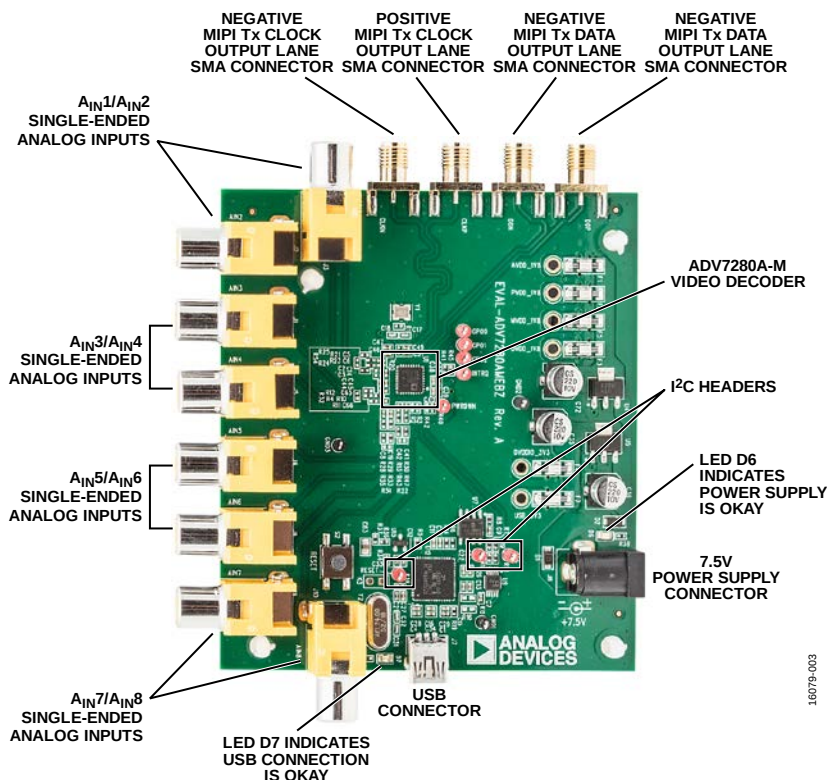
Figure 3. ADV7280A-M Evaluation Board
