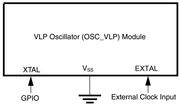
Figure 14-4. External clock connections
