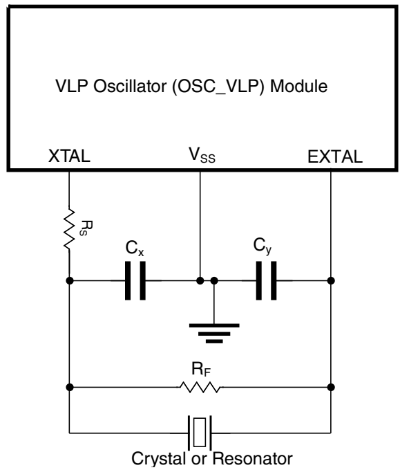
Figure 14-3. Crystal/resonator connections - connection 2
