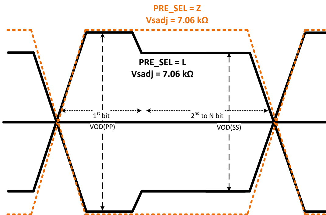
Figure 9. Output De-emphasis Waveform
