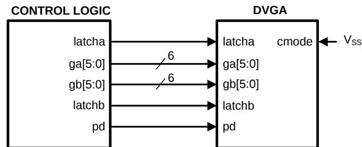
Figure 26. Parallel Mode Connection for Fastest Response
