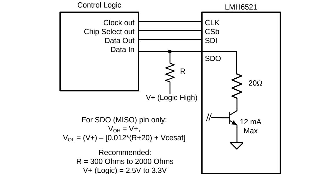
Figure 30. Serial Mode 4-Wire Connection
